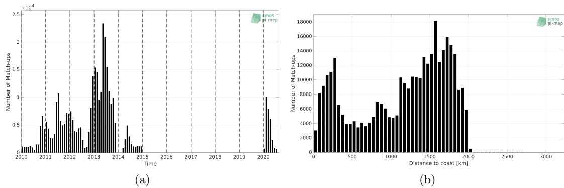
Figure 1: Number of match-ups between Surface drifters and SMOS SSS L3 v335 - Monthly - 25 km (CATDS-CPDC) SSS as a function of time (a) and as function of distance to coast (b) over the Tropical Atlantic Ocean Pi-MEP region and for the full satellite product period.
