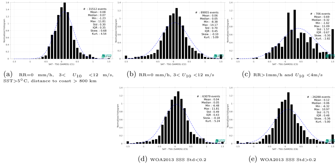
Figure 15: Normalized histogram of \Delta\text{SSS} (SMOS SSS L3 v335 - 10 Days - 25 km (CATDS-CPDC) - TSG (SAMOS)) for 5 different subdatasets corresponding to: RR=0 mm/h, 3 < U_{10} < 12 m/s, SST>5°C, distance to coast > 800 km (a), RR=0 mm/h, 3 < U_{10} < 12 m/s (b), RR>1mm/h and U_{10} < 4 m/s (c), WOA2013 SSS Std<0.2 (d), WOA2013 SSS Std>0.2 (e).
