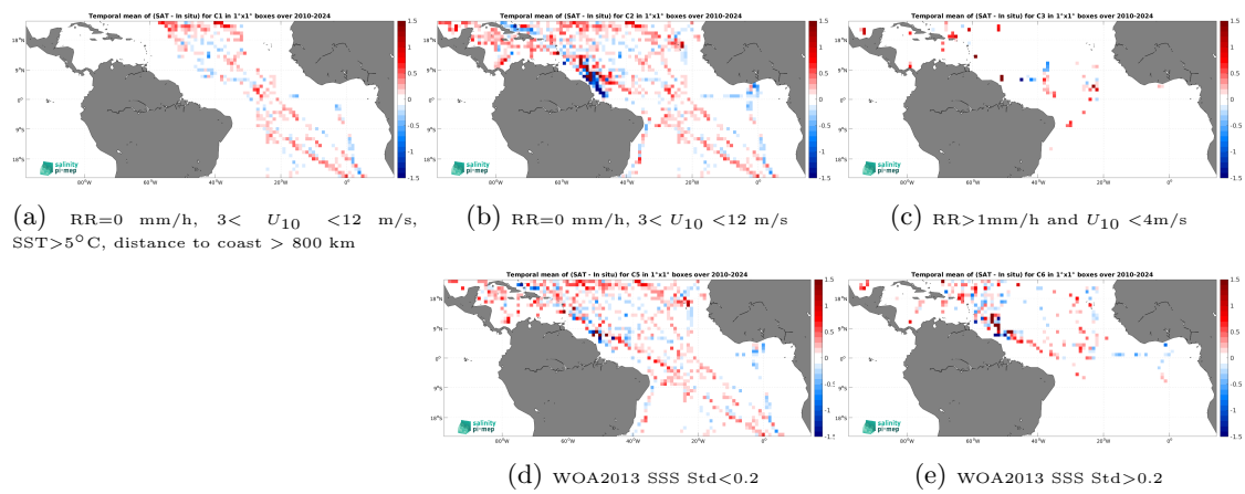
Figure 14: Temporal mean gridded over spatial boxes of size 1^\circ \times 1^\circ of \Delta\text{SSS} (SMOS SSS L3 v335 - 10 Days - 25 km (CATDS-CPDC) - TSG (SAMOS)) for 5 different subdatasets corresponding to:RR=0 mm/h, 3 < U_{10} < 12 m/s, SST>5°C, distance to coast > 800 km (a), RR=0 mm/h, 3 < U_{10} < 12 m/s (b), RR>1mm/h and U_{10} < 4 m/s (c), WOA2013 SSS Std<0.2 (d), WOA2013 SSS Std>0.2 (e).
