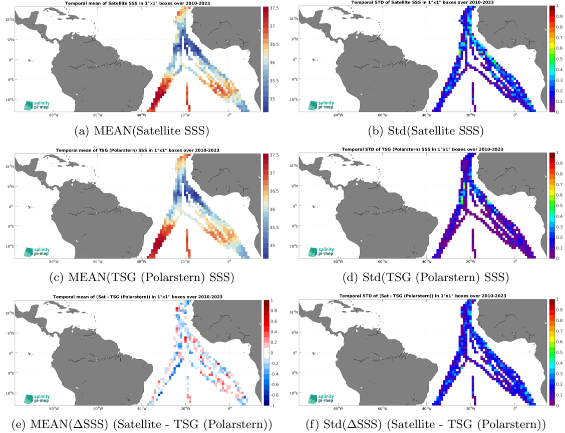
Figure 7: Temporal mean (left) and Std (right) of SSS from SMOS SSS L3 v335 - 10 Days - 25 km (CATDS-CPDC) (top), TSG (Polarstern) (middle), and of \Delta\text{SSS}(\text{Satellite} - \text{TSG}(\text{Polarstern})) . Only match-up pairs are used to generate these maps.
