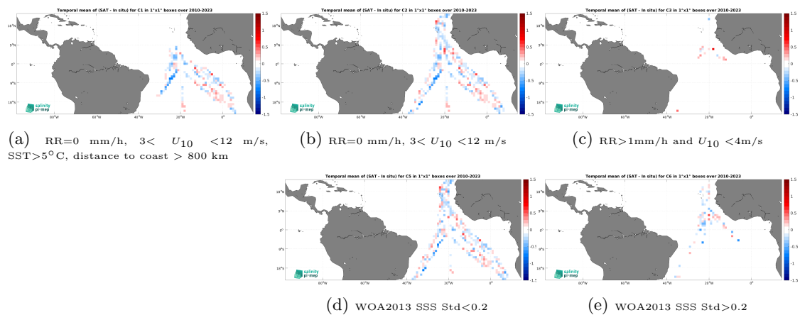
Figure 14: Temporal mean gridded over spatial boxes of size 1^\circ \times 1^\circ of \Delta\text{SSS} (SMOS SSS L3 v335 - 10 Days - 25 km (CATDS-CPDC) - TSG (Polarstern)) for 5 different subdatasets corresponding to:RR=0 mm/h, 3 < U_{10} < 12 m/s, SST>5°C, distance to coast > 800 km (a), RR=0 mm/h, 3 < U_{10} < 12 m/s (b), RR>1mm/h and U_{10} < 4 m/s (c), WOA2013 SSS Std<0.2 (d), WOA2013 SSS Std>0.2 (e).
