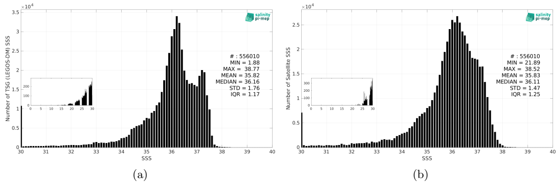
Figure 3: Histograms of SSS from TSG (LEGOS-DM) (a) and SMOS SSS L3 v335 - 10 Days - 25 km (CATDS-CPDC) (b) considering all match-up pairs per bins of 0.1 over the Tropical Atlantic Ocean Pi-MEP region and for the full satellite product period.
