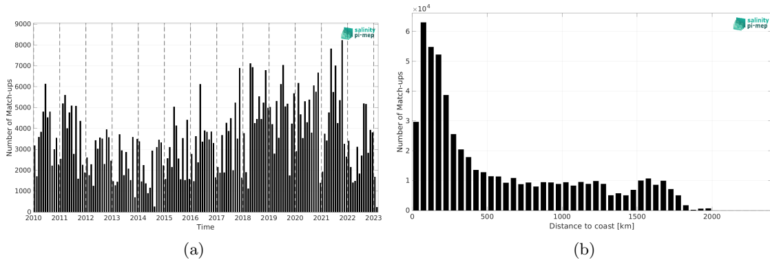
Figure 2: Number of match-ups between TSG (LEGOS-DM) and SMOS SSS L3 v335 - 10 Days - 25 km (CATDS-CPDC) SSS as a function of time (a) and as function of the distance to coast (b) over the Tropical Atlantic Ocean Pi-MEP region and for the full satellite product period.
