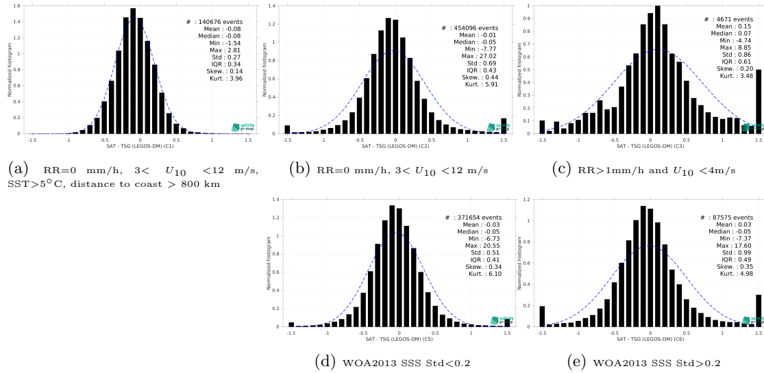
Figure 15: Normalized histogram of \Delta\text{SSS} (SMOS SSS L3 v335 - 10 Days - 25 km (CATDS-CPDC) - TSG (LEGOS-DM)) for 5 different subdatasets corresponding to: RR=0 mm/h, 3 < U_{10} < 12 m/s, SST>5°C, distance to coast > 800 km (a), RR=0 mm/h, 3 < U_{10} < 12 m/s (b), RR>1mm/h and U_{10} < 4 m/s (c), WOA2013 SSS Std<0.2 (d), WOA2013 SSS Std>0.2 (e).
