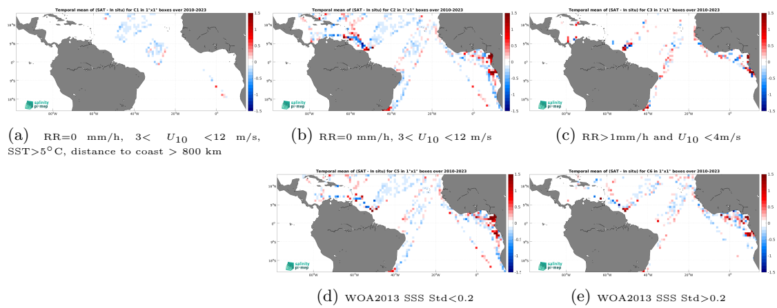
Figure 14: Temporal mean gridded over spatial boxes of size 1^\circ \times 1^\circ of \Delta\text{SSS} (SMOS SSS L3 v335 - 10 Days - 25 km (CATDS-CPDC) - TSG (LEGOS-DM)) for 5 different subdatasets corresponding to:RR=0 mm/h, 3 < U_{10} < 12 m/s, SST>5°C, distance to coast > 800 km (a), RR=0 mm/h, 3 < U_{10} < 12 m/s (b), RR>1mm/h and U_{10} < 4 m/s (c), WOA2013 SSS Std<0.2 (d), WOA2013 SSS Std>0.2 (e).
