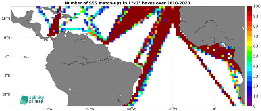
Figure 5: Number of SSS match-ups between TSG (LEGOS-DM) SSS and the SMOS SSS L3 v335 - 10 Days - 25 km (CATDS-CPDC) SSS product for the Tropical Atlantic Ocean Pi-MEP region over 1^\circ \times 1^\circ boxes and for the full satellite product period.
