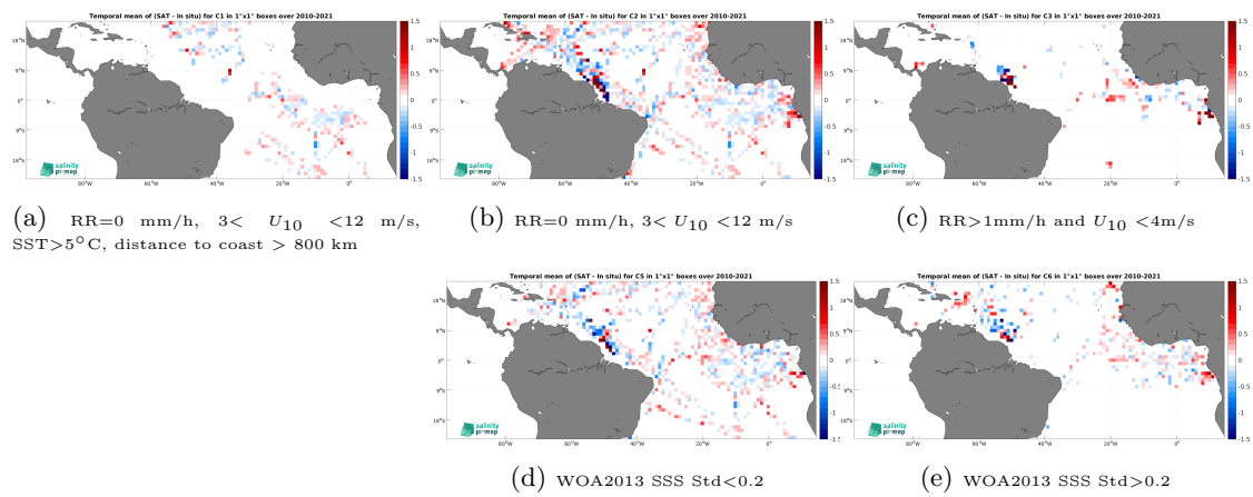
Figure 12: Temporal mean gridded over spatial boxes of size 1^\circ \times 1^\circ of \Delta\text{SSS} (SMOS SSS L3 v335 - 10 Days - 25 km (CATDS-CPDC) - TSG (GOSUD-Research-vessel)) for 5 different subdatasets corresponding to:RR=0 mm/h, 3 < U_{10} < 12 m/s, SST>5°C, distance to coast > 800 km (a), RR=0 mm/h, 3 < U_{10} < 12 m/s (b), RR>1mm/h and U_{10} < 4 m/s (c), WOA2013 SSS Std<0.2 (d), WOA2013 SSS Std>0.2 (e).
