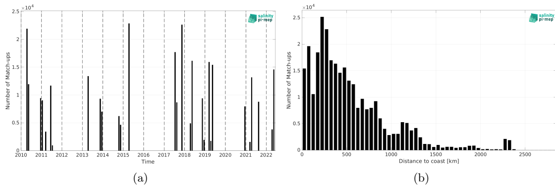
Figure 2: Number of match-ups between TSG (CSIC-UTM) and SMOS SSS L3 v335 - 10 Days - 25 km (CATDS-CPDC) SSS as a function of time (a) and as function of the distance to coast (b) over the Tropical Atlantic Ocean Pi-MEP region and for the full satellite product period.
