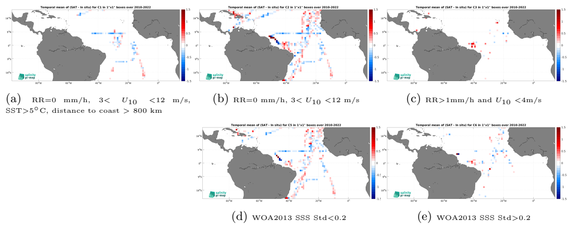
Figure 14: Temporal mean gridded over spatial boxes of size 1^\circ \times 1^\circ of \Delta SSS (SMOS SSS L3 v335 - 10 Days - 25 km (CATDS-CPDC) - TSG (CSIC-UTM)) for 5 different subdatasets corresponding to:RR=0 mm/h, 3 < U_{10} < 12 m/s, SST >5^\circ\text{C} , distance to coast > 800 km (a), RR=0 mm/h, 3 < U_{10} < 12 m/s (b), RR >1 mm/h and U_{10} < 4 m/s (c), WOA2013 SSS Std <0.2 (d), WOA2013 SSS Std >0.2 (e).
