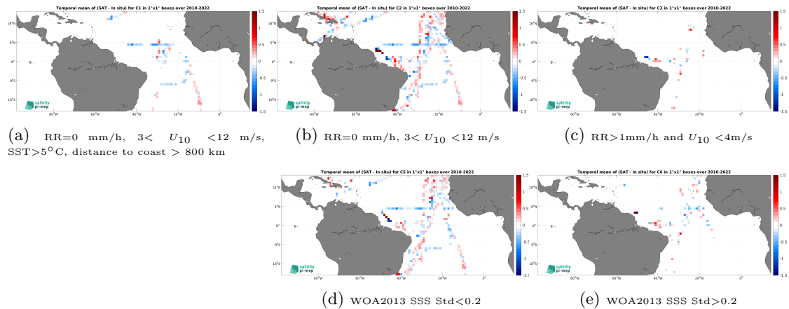
Figure 12: Temporal mean gridded over spatial boxes of size 1^\circ \times 1^\circ of \Delta\text{SSS} (SMOS SSS L3 v335 - 10 Days - 25 km (CATDS-CPDC) - TSG (CSIC-UTM)) for 5 different subdatasets corresponding to:RR=0 mm/h, 3 < U_{10} < 12 m/s, SST >5^\circ\text{C} , distance to coast > 800 km (a), RR=0 mm/h, 3 < U_{10} < 12 m/s (b), RR >1 mm/h and U_{10} < 4 m/s (c), WOA2013 SSS Std <0.2 (d), WOA2013 SSS Std >0.2 (e).
