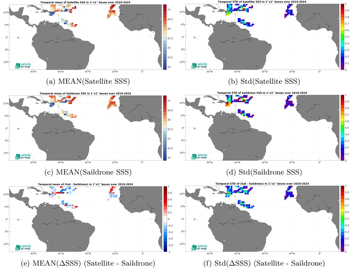
Figure 7: Temporal mean (left) and Std (right) of SSS from SMOS SSS L3 v335 - 10 Days - 25 km (CATDS-CPDC) (top), Sairdrone (middle), and of \Delta SSS (Satellite - Sairdrone). Only match-up pairs are used to generate these maps.
