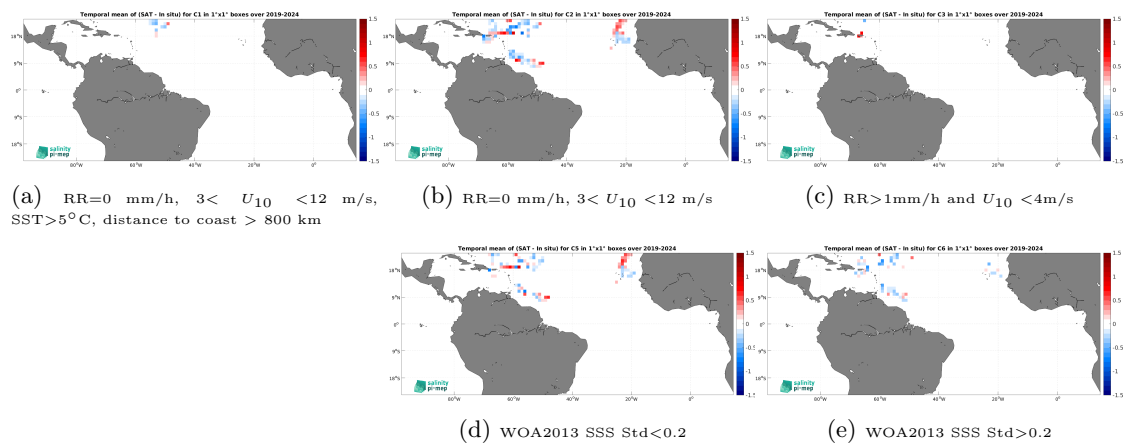
Figure 14: Temporal mean gridded over spatial boxes of size 1^\circ \times 1^\circ of \Delta\text{SSS} (SMOS SSS L3 v335 - 10 Days - 25 km (CATDS-CPDC) - Saildrone) for 5 different subdatasets corresponding to:RR=0 mm/h, 3 < U_{10} < 12 m/s, SST>5°C, distance to coast > 800 km (a), RR=0 mm/h, 3 < U_{10} < 12 m/s (b), RR>1mm/h and U_{10} < 4 m/s (c), WOA2013 SSS Std<0.2 (d), WOA2013 SSS Std>0.2 (e).
