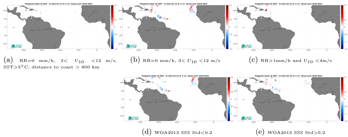
Figure 14: Temporal mean gridded over spatial boxes of size 1^\circ \times 1^\circ of \Delta\text{SSS} (SMOS SSS L3 v335 - 10 Days - 25 km (CATDS-CPDC) - Saildrone) for 5 different subdatasets corresponding to:RR=0 mm/h, 3 < U_{10} < 12 m/s, SST>5°C, distance to coast > 800 km (a), RR=0 mm/h, 3 < U_{10} < 12 m/s (b), RR>1mm/h and U_{10} < 4 m/s (c), WOA2013 SSS Std<0.2 (d), WOA2013 SSS Std>0.2 (e).
