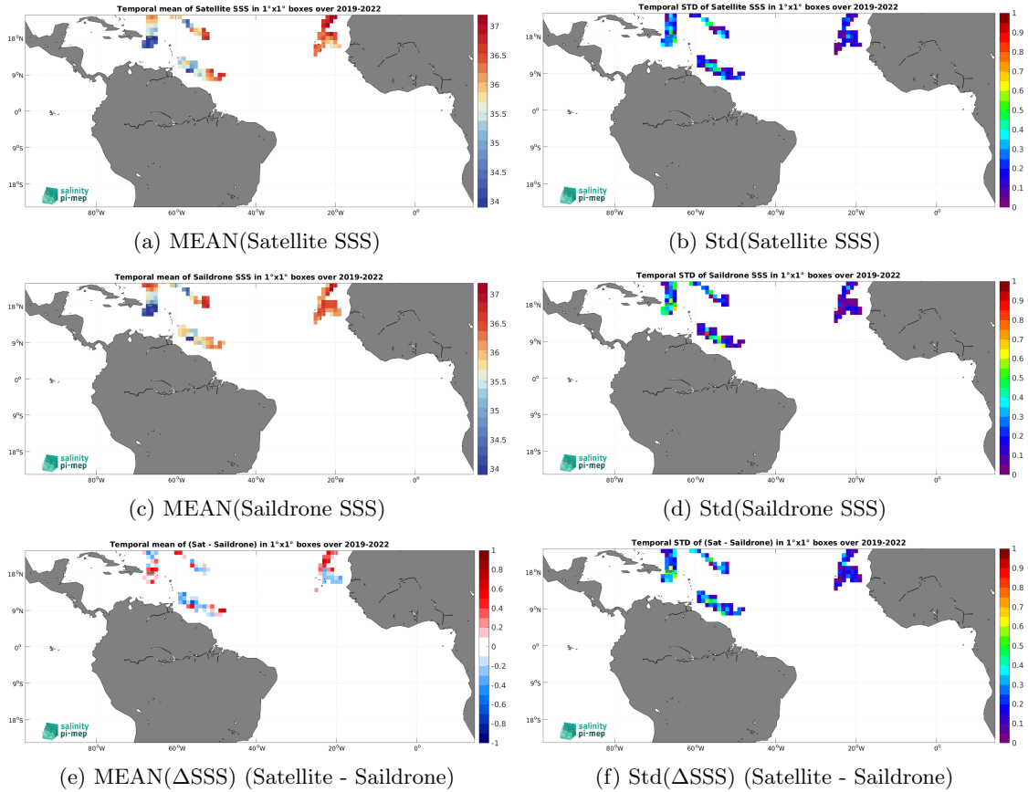
Figure 7: Temporal mean (left) and Std (right) of SSS from SMOS SSS L3 v335 - 10 Days - 25 km (CATDS-CPDC) (top), Sairdron (middle), and of \Delta SSS (Satellite - Sairdron). Only match-up pairs are used to generate these maps.
