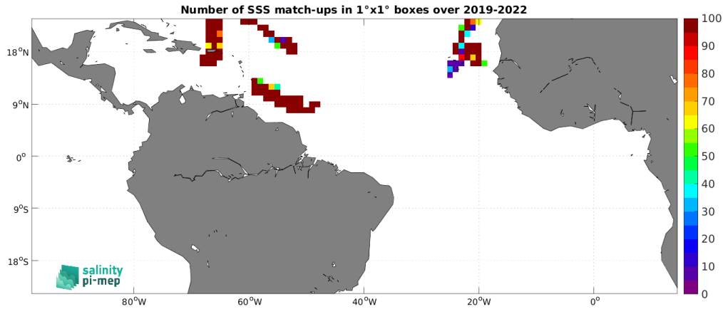
Figure 5: Number of SSS match-ups between Saildrone SSS and the SMOS SSS L3 v335 - 10 Days - 25 km (CATDS-CPDC) SSS product for the Tropical Atlantic Ocean Pi-MEP region over 1^\circ \times 1^\circ boxes and for the full satellite product period.
