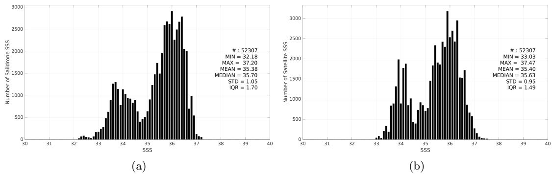
Figure 3: Histograms of SSS from Saildrone (a) and SMOS SSS L3 v335 - 10 Days - 25 km (CATDS-CPDC) (b) considering all match-up pairs per bins of 0.1 over the Tropical Atlantic Ocean Pi-MEP region and for the full satellite product period.
