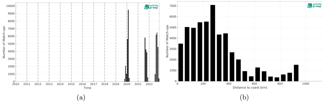
Figure 2: Number of match-ups between Saildrone and SMOS SSS L3 v335 - 10 Days - 25 km (CATDS-CPDC) SSS as a function of time (a) and as function of the distance to coast (b) over the Tropical Atlantic Ocean Pi-MEP region and for the full satellite product period.
