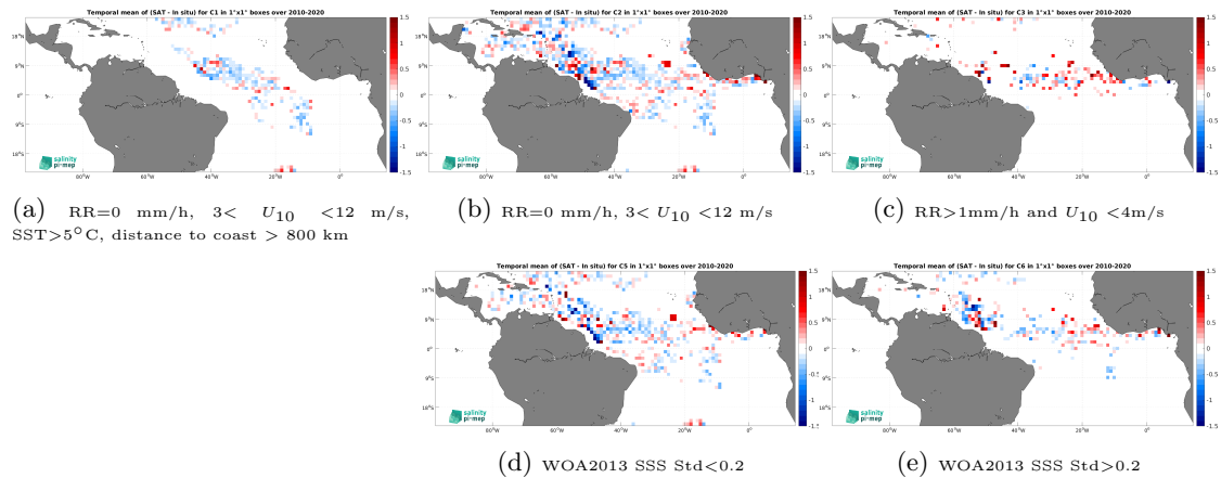
Figure 13: Temporal mean gridded over spatial boxes of size 1^\circ \times 1^\circ of \Delta\text{SSS} (SMOS SSS L3 v335 - 10 Days - 25 km (CATDS-CPDC) - Surface drifters) for 5 different subdatasets corresponding to:RR=0 mm/h, 3 < U_{10} < 12 m/s, SST >5^\circ\text{C} , distance to coast > 800 km (a), RR=0 mm/h, 3 < U_{10} < 12 m/s (b), RR >1 mm/h and U_{10} < 4 m/s (c), WOA2013 SSS Std <0.2 (d), WOA2013 SSS Std >0.2 (e).
