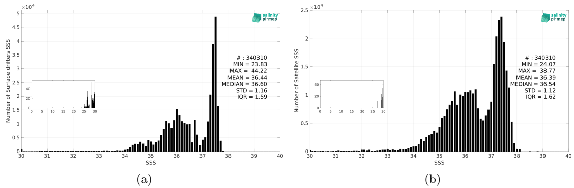
Figure 3: Histograms of SSS from Surface drifters (a) and SMOS SSS L3 v335 - 10 Days - 25 km (CATDS-CPDC) (b) considering all match-up pairs per bins of 0.1 over the Tropical Atlantic Ocean Pi-MEP region and for the full satellite product period.
