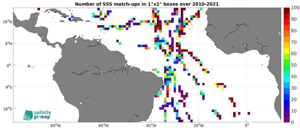
Figure 5: Number of SSS match-ups between TSG (GOSUD-Sailing-ship) SSS and the SMOS SSS L2Q v333 - 0.25 Deg (CATDS-CPDC) SSS product for the Tropical Atlantic Ocean Pi-MEP region over 1^\circ \times 1^\circ boxes and for the full satellite product period.
