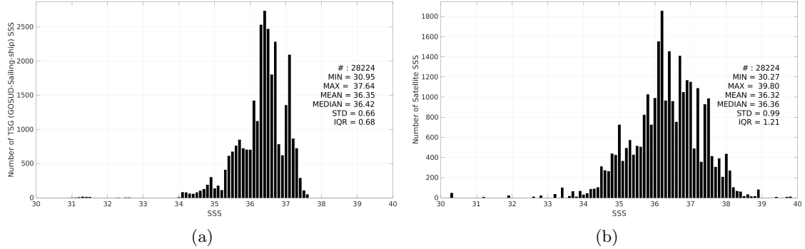
Figure 3: Histograms of SSS from TSG (GOSUD-Sailing-ship) (a) and SMOS SSS L2Q v333 - 0.25 Deg (CATDS-CPDC) (b) considering all match-up pairs per bins of 0.1 over the Tropical Atlantic Ocean Pi-MEP region and for the full satellite product period.
