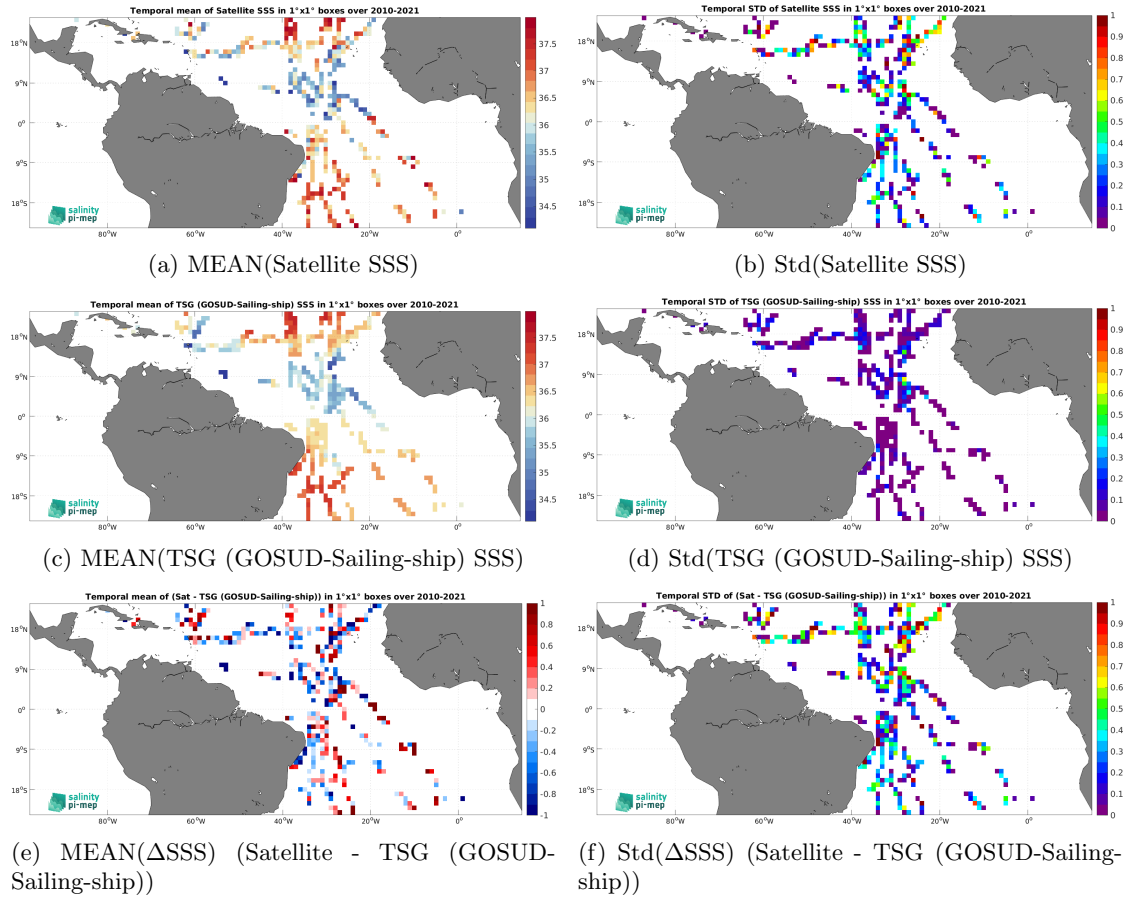
Figure 7: Temporal mean (left) and Std (right) of SSS from SMOS SSS L2Q v333 - 0.25 Deg (CATDS-CPDC) (top), TSG (GOSUD-Sailing-ship) (middle), and of \Delta\text{SSS} (Satellite - TSG (GOSUD-Sailing-ship)). Only match-up pairs are used to generate these maps.
