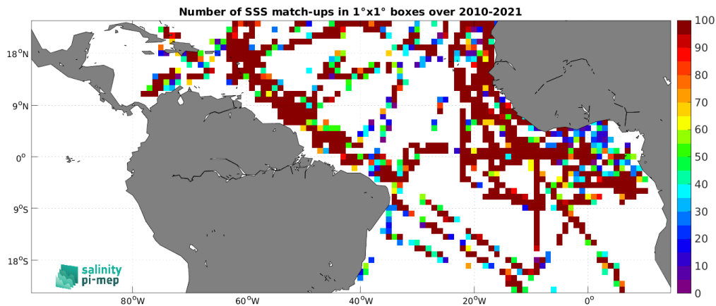
Figure 5: Number of SSS match-ups between TSG (GOSUD-Research-vessel) SSS and the SMOS SSS L2Q v333 - 0.25 Deg (CATDS-CPDC) SSS product for the Tropical Atlantic Ocean Pi-MEP region over 1°×1° boxes and for the full satellite product period.
