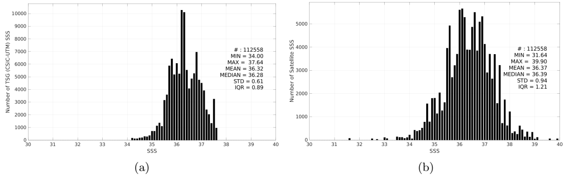
Figure 3: Histograms of SSS from TSG (CSIC-UTM) (a) and SMOS SSS L2Q v333 - 0.25 Deg (CATDS-CPDC) (b) considering all match-up pairs per bins of 0.1 over the Tropical Atlantic Ocean Pi-MEP region and for the full satellite product period.
