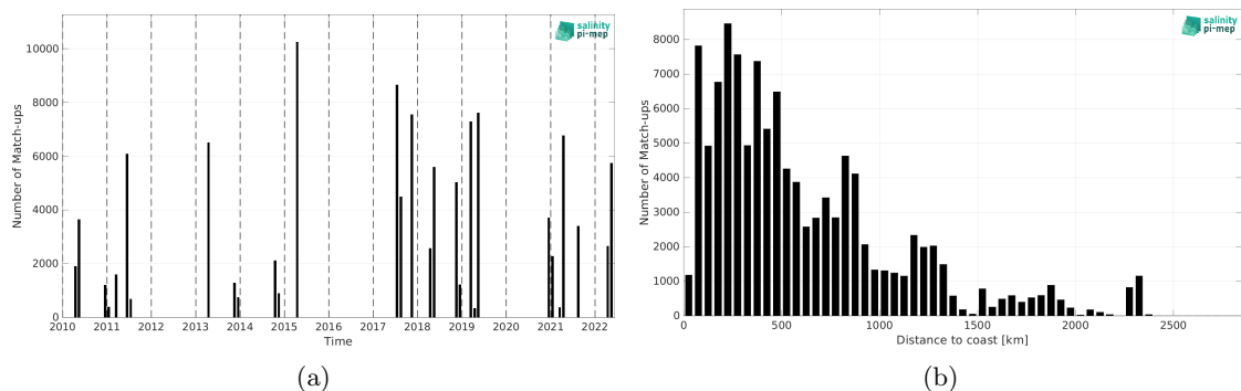
Figure 2: Number of match-ups between TSG (CSIC-UTM) and SMOS SSS L2Q v333 - 0.25 Deg (CATDS-CPDC) SSS as a function of time (a) and as function of the distance to coast (b) over the Tropical Atlantic Ocean Pi-MEP region and for the full satellite product period.
