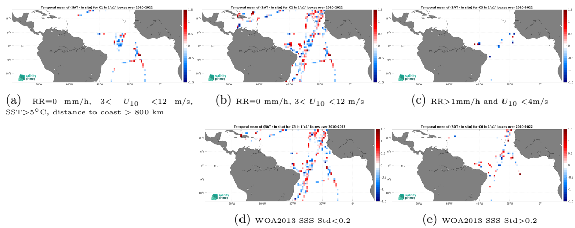
Figure 14: Temporal mean gridded over spatial boxes of size 1^\circ \times 1^\circ of \Delta SSS (SMOS SSS L2Q v333 - 0.25 Deg (CATDS-CPDC) - TSG (CSIC-UTM)) for 5 different subdatasets corresponding to:RR=0 mm/h, 3 < U_{10} < 12 m/s, SST >5^\circ\text{C} , distance to coast > 800 km (a), RR=0 mm/h, 3 < U_{10} < 12 m/s (b), RR >1 mm/h and U_{10} < 4 m/s (c), WOA2013 SSS Std <0.2 (d), WOA2013 SSS Std >0.2 (e).
