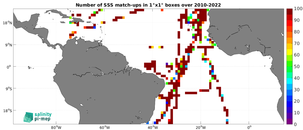
Figure 5: Number of SSS match-ups between TSG (CSIC-UTM) SSS and the SMOS SSS L2Q v333 - 0.25 Deg (CATDS-CPDC) SSS product for the Tropical Atlantic Ocean Pi-MEP region over 1^\circ \times 1^\circ boxes and for the full satellite product period.
