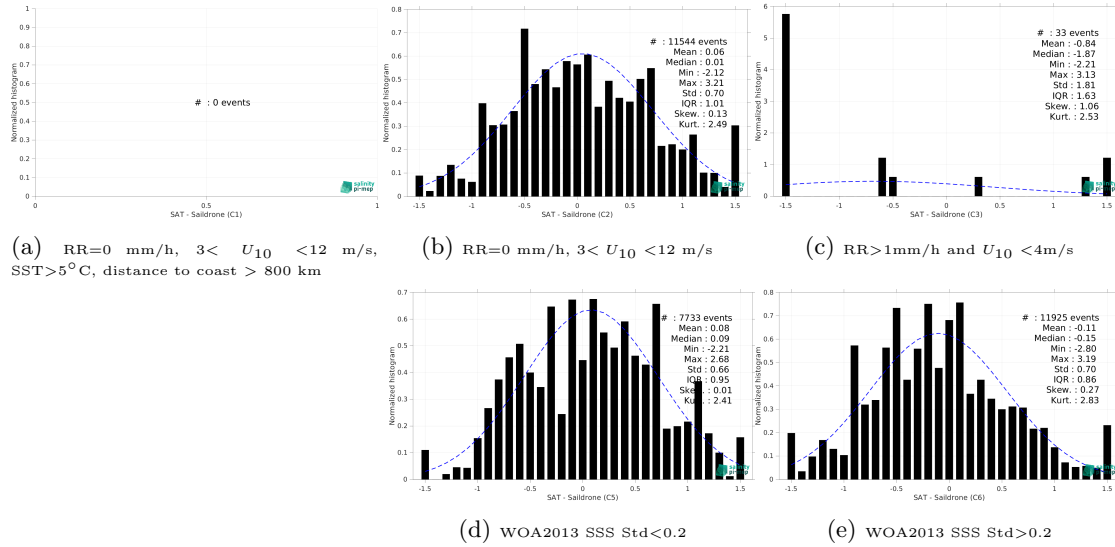
Figure 15: Normalized histogram of \Delta SSS (SMOS SSS L2Q v333 - 0.25 Deg (CATDS-CPDC) - Saldrone) for 5 different subdatasets corresponding to: RR=0 mm/h, 3 < U_{10} < 12 m/s, SST>5°C, distance to coast > 800 km (a), RR=0 mm/h, 3 < U_{10} < 12 m/s (b), RR>1mm/h and U_{10} < 4 m/s (c), WOA2013 SSS Std<0.2 (d), WOA2013 SSS Std>0.2 (e).
