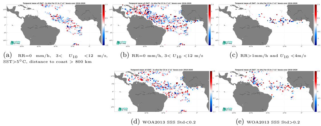
Figure 13: Temporal mean gridded over spatial boxes of size 1^\circ \times 1^\circ of \Delta\text{SSS} (SMOS SSS L2Q v333 - 0.25 Deg (CATDS-CPDC) - Surface drifters) for 5 different subdatasets corresponding to:RR=0 mm/h, 3 < U_{10} < 12 m/s, SST >5^\circ\text{C} , distance to coast > 800 km (a), RR=0 mm/h, 3 < U_{10} < 12 m/s (b), RR >1 mm/h and U_{10} < 4 m/s (c), WOA2013 SSS Std <0.2 (d), WOA2013 SSS Std >0.2 (e).
