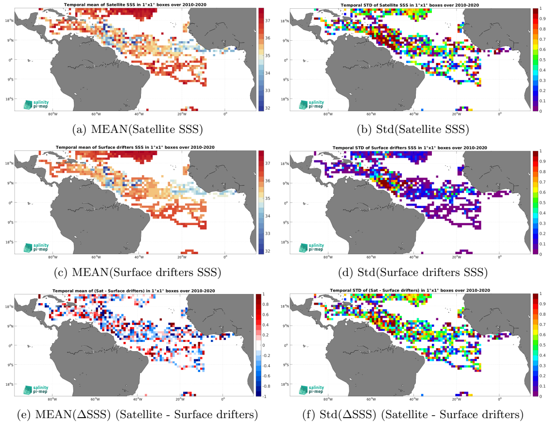
Figure 6: Temporal mean (left) and Std (right) of SSS from SMOS SSS L2Q v333 - 0.25 Deg (CATDS-CPDC) (top), Surface drifters (middle), and of \Delta SSS (Satellite - Surface drifters). Only match-up pairs are used to generate these maps.
