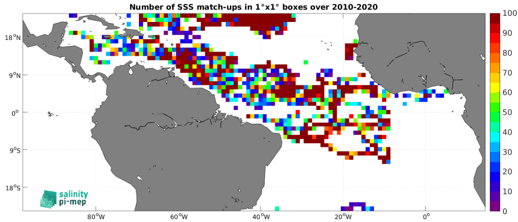
Figure 4: Number of SSS match-ups between Surface drifters SSS and the SMOS SSS L2Q v333 - 0.25 Deg (CATDS-CPDC) SSS product for the Tropical Atlantic Ocean Pi-MEP region over 1^\circ \times 1^\circ boxes and for the full satellite product period.
