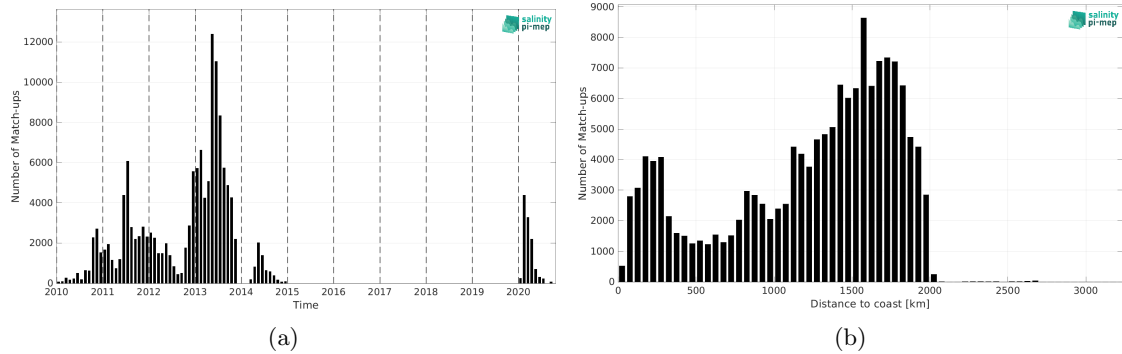
Figure 2: Number of match-ups between Surface drifters and SMOS SSS L2Q v333 - 0.25 Deg (CATDS-CPDC) SSS as a function of time (a) and as function of the distance to coast (b) over the Tropical Atlantic Ocean Pi-MEP region and for the full satellite product period.
