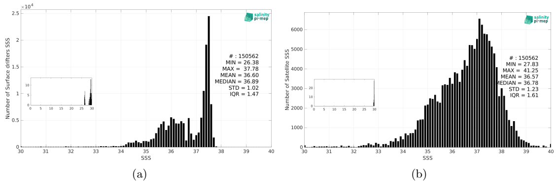
Figure 3: Histograms of SSS from Surface drifters (a) and SMOS SSS L2Q v333 - 0.25 Deg (CATDS-CPDC) (b) considering all match-up pairs per bins of 0.1 over the Tropical Atlantic Ocean Pi-MEP region and for the full satellite product period.
