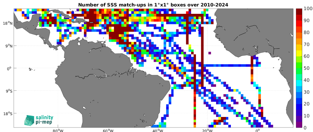
Figure 5: Number of SSS match-ups between TSG (SAMOS) SSS and the SMOS SSS L3 v332 - 9 Days (CATDS-CPDC) SSS product for the Tropical Atlantic Ocean Pi-MEP region over 1^\circ \times 1^\circ boxes and for the full satellite product period.
