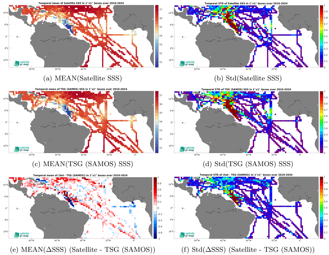
Figure 7: Temporal mean (left) and Std (right) of SSS from SMOS SSS L3 v332 - 9 Days (CATDS-CPDC) (top), TSG (SAMOS) (middle), and of \Delta SSS (Satellite - TSG (SAMOS)). Only match-up pairs are used to generate these maps.
