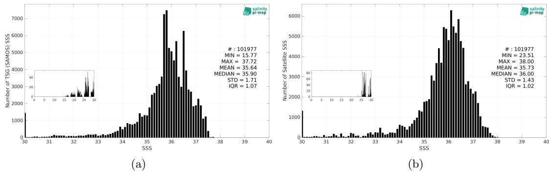
Figure 3: Histograms of SSS from TSG (SAMOS) (a) and SMOS SSS L3 v332 - 9 Days (CATDS-CPDC) (b) considering all match-up pairs per bins of 0.1 over the Tropical Atlantic Ocean Pi-MEP region and for the full satellite product period.
