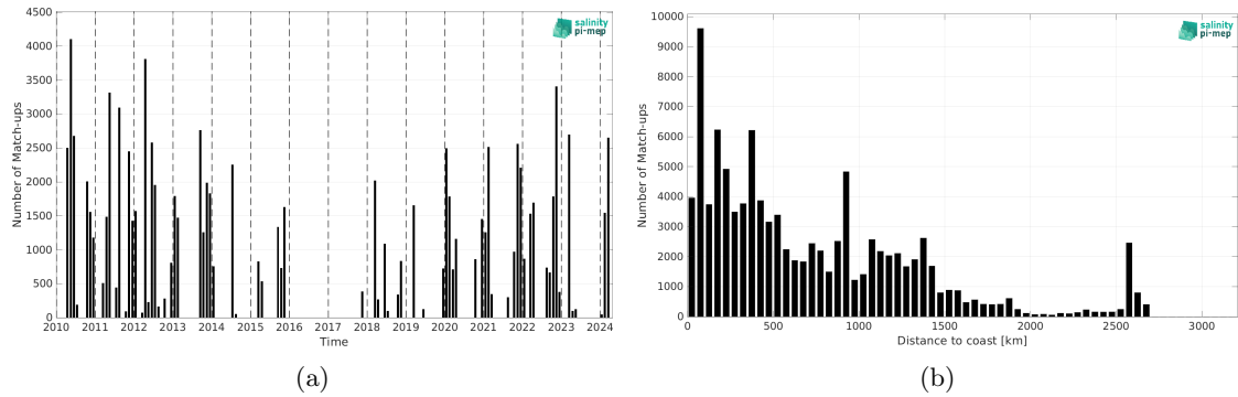
Figure 2: Number of match-ups between TSG (SAMOS) and SMOS SSS L3 v332 - 9 Days (CATDS-CPDC) SSS as a function of time (a) and as function of the distance to coast (b) over the Tropical Atlantic Ocean Pi-MEP region and for the full satellite product period.
