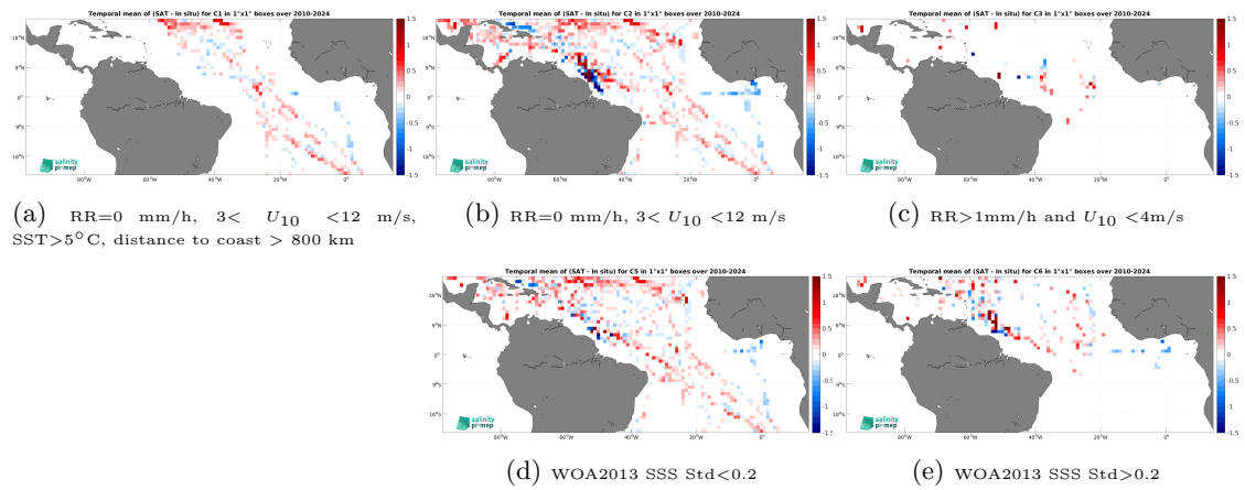
Figure 14: Temporal mean gridded over spatial boxes of size 1^\circ \times 1^\circ of \Delta SSS (SMOS SSS L3 v332 - 9 Days (CATDS-CPDC) - TSG (SAMOS)) for 5 different subdatasets corresponding to:RR=0 mm/h, 3 < U_{10} < 12 m/s, SST>5°C, distance to coast > 800 km (a), RR=0 mm/h, 3 < U_{10} < 12 m/s (b), RR>1mm/h and U_{10} < 4 m/s (c), WOA2013 SSS Std<0.2 (d), WOA2013 SSS Std>0.2 (e).
