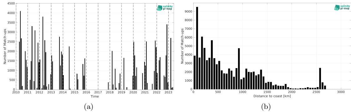
Figure 1: Number of match-ups between TSG (SAMOS) and SMOS SSS L3 v332 - 9 Days (CATDS-CPDC) SSS as a function of time (a) and as function of the distance to coast (b) over the Tropical Atlantic Ocean Pi-MEP region and for the full satellite product period.
