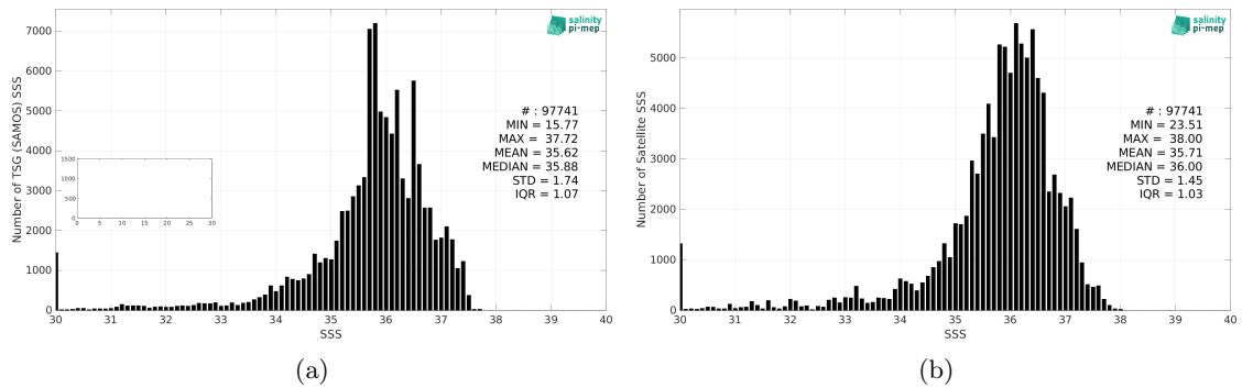
Figure 2: Histograms of SSS from TSG (SAMOS) (a) and SMOS SSS L3 v332 - 9 Days (CATDS-CPDC) (b) considering all match-up pairs per bins of 0.1 over the Tropical Atlantic Ocean Pi-MEP region and for the full satellite product period.
