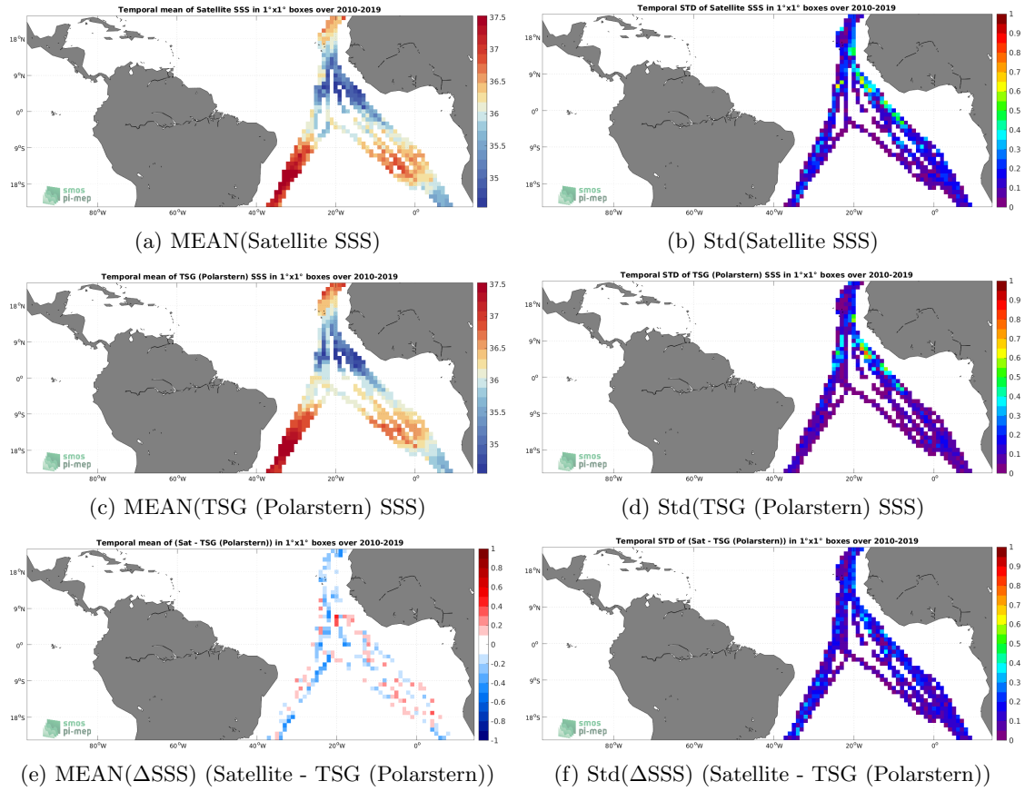
Figure 6: Temporal mean (left) and Std (right) of SSS from SMOS SSS L3 v332 - 9 Days (CATDS-CPDC) (top), TSG (Polarstern) (middle), and of \Delta SSS (Satellite - TSG (Polarstern)). Only match-up pairs are used to generate these maps.
