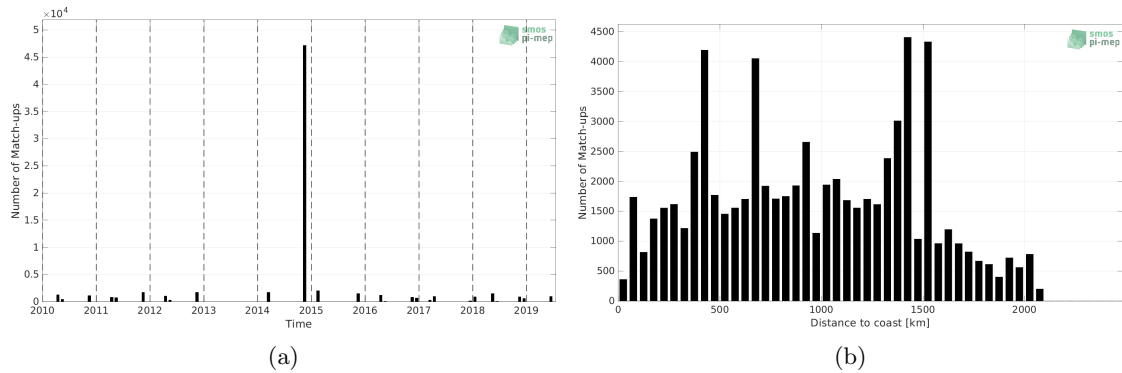
Figure 1: Number of match-ups between TSG (Polarstern) and SMOS SSS L3 v332 - 9 Days (CATDS-CPDC) SSS as a function of time (a) and as function of the distance to coast (b) over the Tropical Atlantic Ocean Pi-MEP region and for the full satellite product period.
