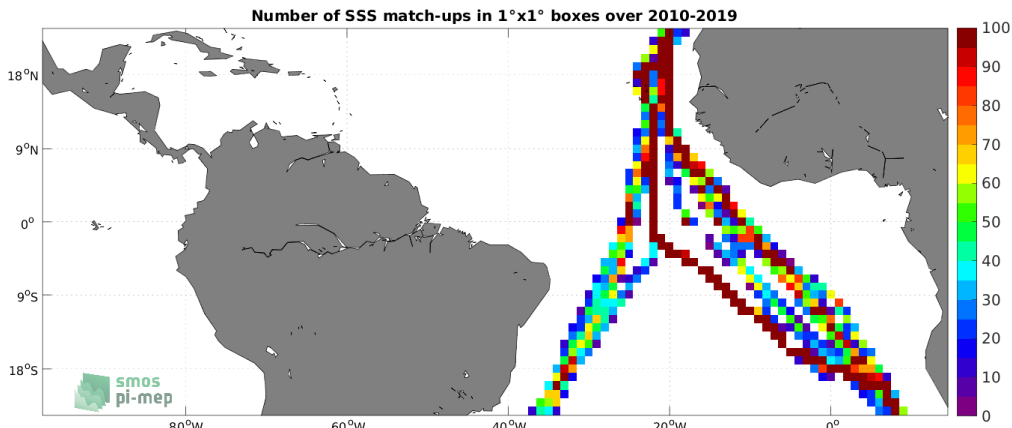
Figure 4: Number of SSS match-ups between TSG (Polarstern) SSS and the SMOS SSS L3 v332 - 9 Days (CATDS-CPDC) SSS product for the Tropical Atlantic Ocean Pi-MEP region over 1^\circ \times 1^\circ boxes and for the full satellite product period.
