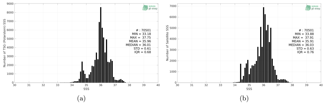
Figure 2: Histograms of SSS from TSG (Polarstern) (a) and SMOS SSS L3 v332 - 9 Days (CATDS-CPDC) (b) considering all match-up pairs per bins of 0.1 over the Tropical Atlantic Ocean Pi-MEP region and for the full satellite product period.
