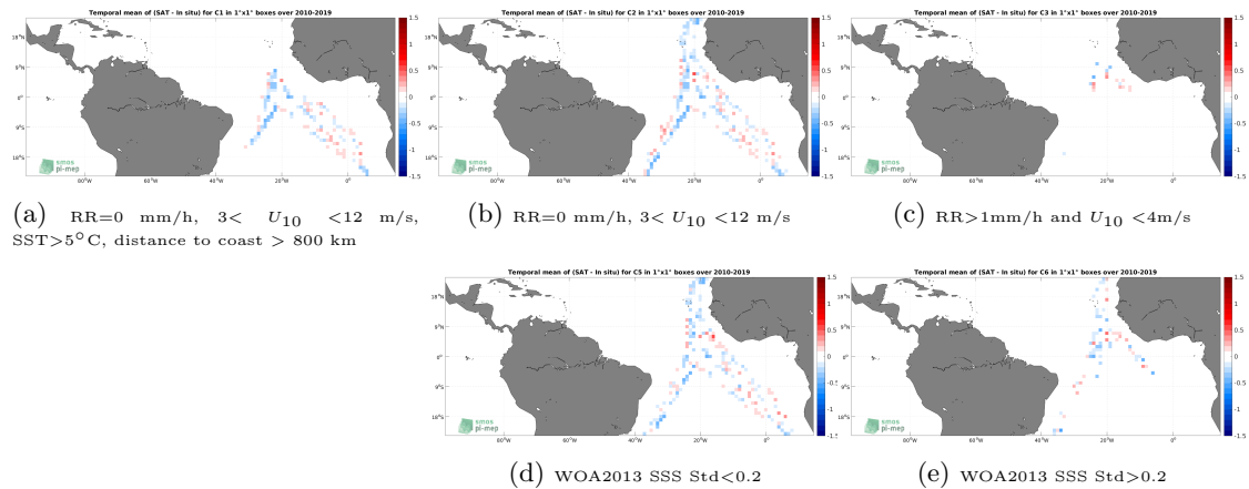
Figure 12: Temporal mean gridded over spatial boxes of size 1^\circ \times 1^\circ of \Delta\text{SSS} (SMOS SSS L3 v332 - 9 Days (CATDS-CPDC) - TSG (Polarstern)) for 5 different subdatasets corresponding to:RR=0 mm/h, 3 < U_{10} < 12 m/s, SST >5^\circ\text{C} , distance to coast > 800 km (a), RR=0 mm/h, 3 < U_{10} < 12 m/s (b), RR >1 mm/h and U_{10} < 4 m/s (c), WOA2013 SSS Std <0.2 (d), WOA2013 SSS Std >0.2 (e).
