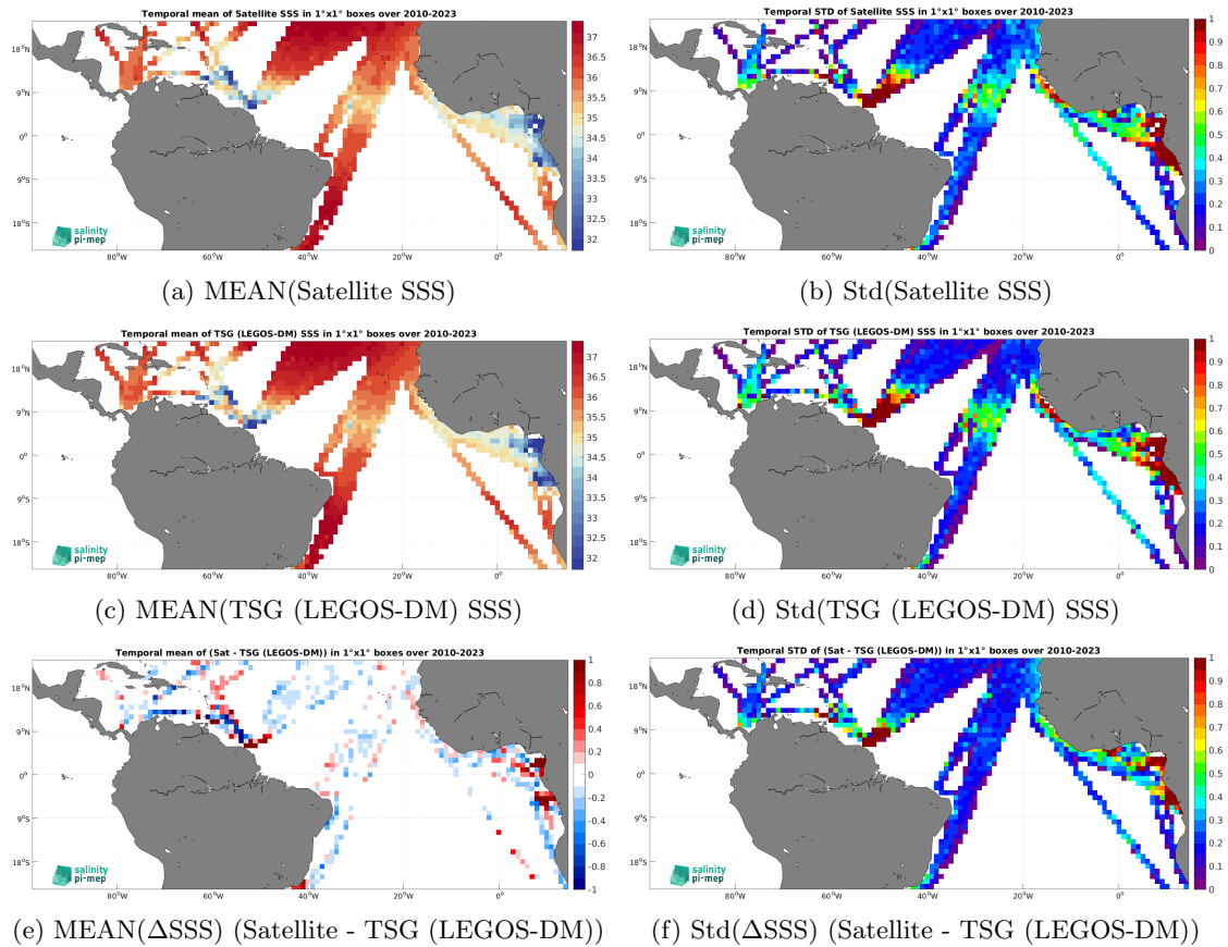
Figure 7: Temporal mean (left) and Std (right) of SSS from SMOS SSS L3 v332 - 9 Days (CATDS-CPDC) (top), TSG (LEGOS-DM) (middle), and of \Delta SSS (Satellite - TSG (LEGOS-DM)). Only match-up pairs are used to generate these maps.
