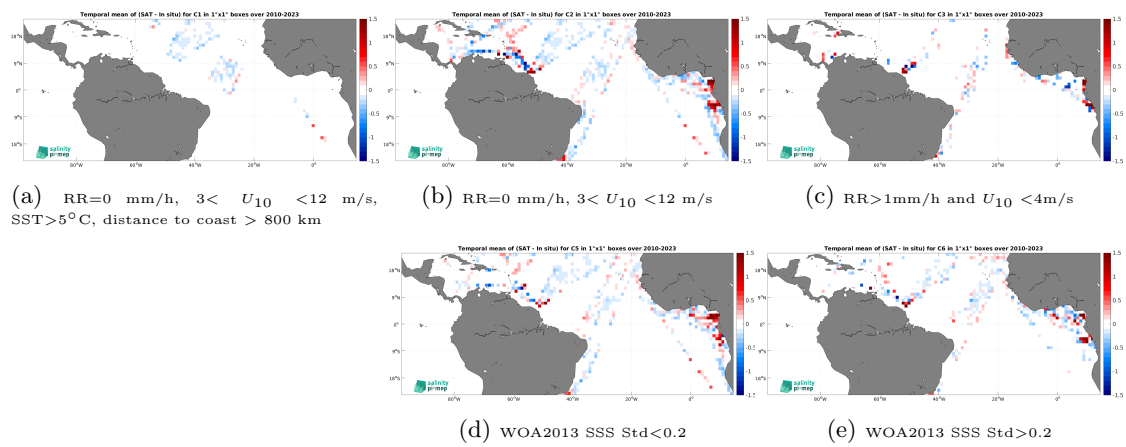
Figure 14: Temporal mean gridded over spatial boxes of size 1^\circ \times 1^\circ of \Delta\text{SSS} (SMOS SSS L3 v332 - 9 Days (CATDS-CPDC) - TSG (LEGOS-DM)) for 5 different subdatasets corresponding to:RR=0 mm/h, 3 < U_{10} < 12 m/s, SST>5°C, distance to coast > 800 km (a), RR=0 mm/h, 3 < U_{10} < 12 m/s (b), RR>1mm/h and U_{10} < 4 m/s (c), WOA2013 SSS Std<0.2 (d), WOA2013 SSS Std>0.2 (e).
