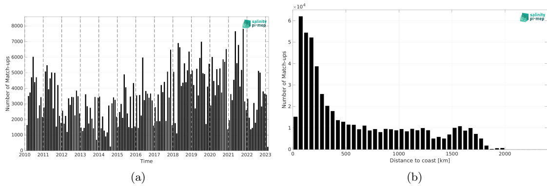
Figure 2: Number of match-ups between TSG (LEGOS-DM) and SMOS SSS L3 v332 - 9 Days (CATDS-CPDC) SSS as a function of time (a) and as function of the distance to coast (b) over the Tropical Atlantic Ocean Pi-MEP region and for the full satellite product period.
