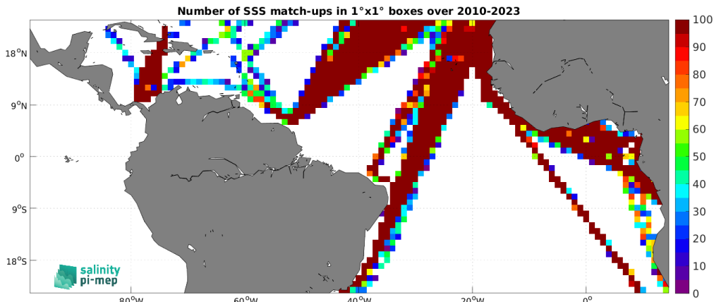
Figure 5: Number of SSS match-ups between TSG (LEGOS-DM) SSS and the SMOS SSS L3 v332 - 9 Days (CATDS-CPDC) SSS product for the Tropical Atlantic Ocean Pi-MEP region over 1^\circ \times 1^\circ boxes and for the full satellite product period.
