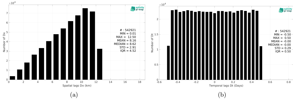
Figure 6: Histograms of the spatial (a) and temporal (b) lags between the location/time of the TSG (LEGOS-DM) measurement and the date of the corresponding SMOS SSS L3 v332 - 9 Days (CATDS-CPDC) SSS pixel.
