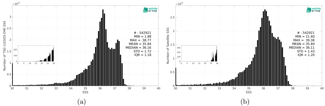
Figure 3: Histograms of SSS from TSG (LEGOS-DM) (a) and SMOS SSS L3 v332 - 9 Days (CATDS-CPDC) (b) considering all match-up pairs per bins of 0.1 over the Tropical Atlantic Ocean Pi-MEP region and for the full satellite product period.
