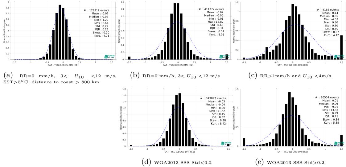
Figure 15: Normalized histogram of \Delta SSS (SMOS SSS L3 v332 - 9 Days (CATDS-CPDC) - TSG (LEGOS-DM)) for 5 different subdatasets corresponding to: RR=0 mm/h, 3 < U_{10} < 12 m/s, SST > 5°C, distance to coast > 800 km (a), RR=0 mm/h, 3 < U_{10} < 12 m/s (b), RR > 1mm/h and U_{10} < 4 m/s (c), WOA2013 SSS Std < 0.2 (d), WOA2013 SSS Std > 0.2 (e).
