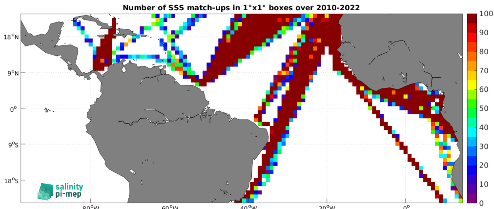
Figure 4: Number of SSS match-ups between TSG (LEGOS-DM) SSS and the SMOS SSS L3 v332 - 9 Days (CATDS-CPDC) SSS product for the Tropical Atlantic Ocean Pi-MEP region over 1^\circ \times 1^\circ boxes and for the full satellite product period.
