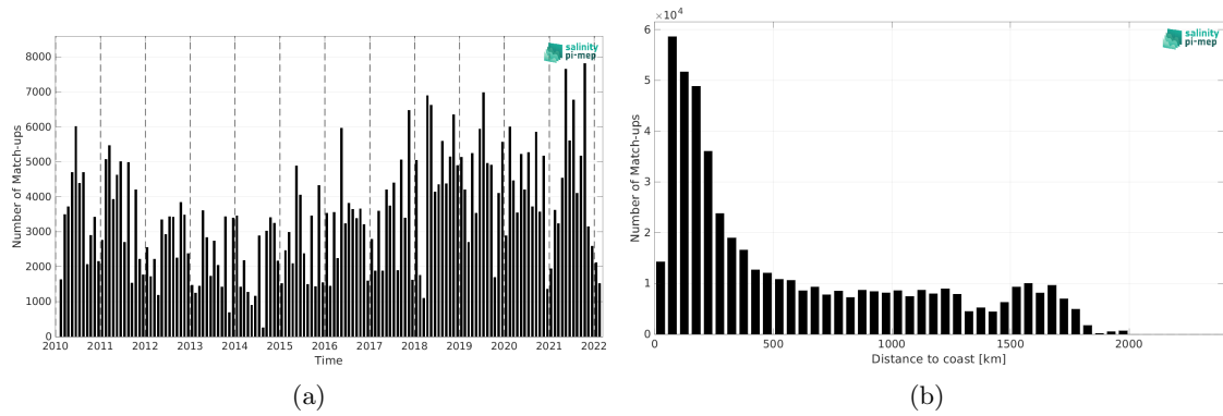
Figure 1: Number of match-ups between TSG (LEGOS-DM) and SMOS SSS L3 v332 - 9 Days (CATDS-CPDC) SSS as a function of time (a) and as function of the distance to coast (b) over the Tropical Atlantic Ocean Pi-MEP region and for the full satellite product period.
