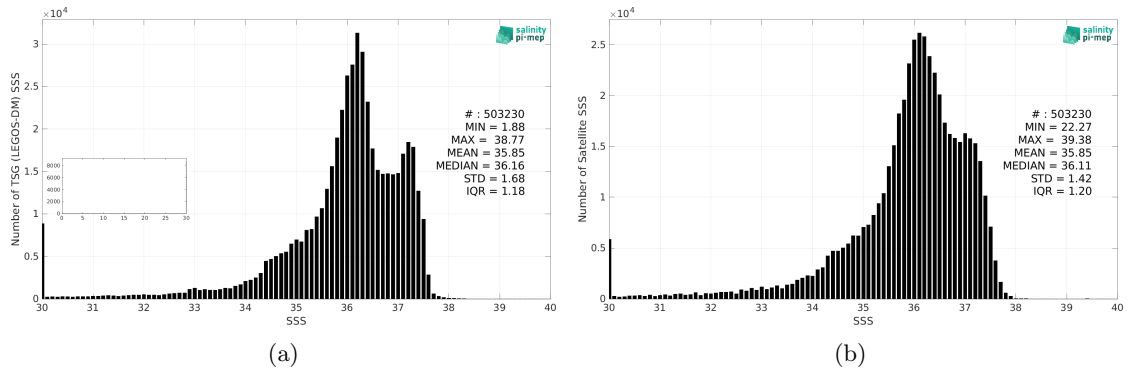
Figure 2: Histograms of SSS from TSG (LEGOS-DM) (a) and SMOS SSS L3 v332 - 9 Days (CATDS-CPDC) (b) considering all match-up pairs per bins of 0.1 over the Tropical Atlantic Ocean Pi-MEP region and for the full satellite product period.
