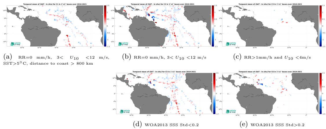
Figure 14: Temporal mean gridded over spatial boxes of size 1^\circ \times 1^\circ of \Delta SSS (SMOS SSS L3 v332 - 9 Days (CATDS-CPDC) - TSG (GOSUD-Sailing-ship)) for 5 different subdatasets corresponding to:RR=0 mm/h, 3 < U_{10} < 12 m/s, SST>5°C, distance to coast > 800 km (a), RR=0 mm/h, 3 < U_{10} < 12 m/s (b), RR>1mm/h and U_{10} < 4 m/s (c), WOA2013 SSS Std<0.2 (d), WOA2013 SSS Std>0.2 (e).
