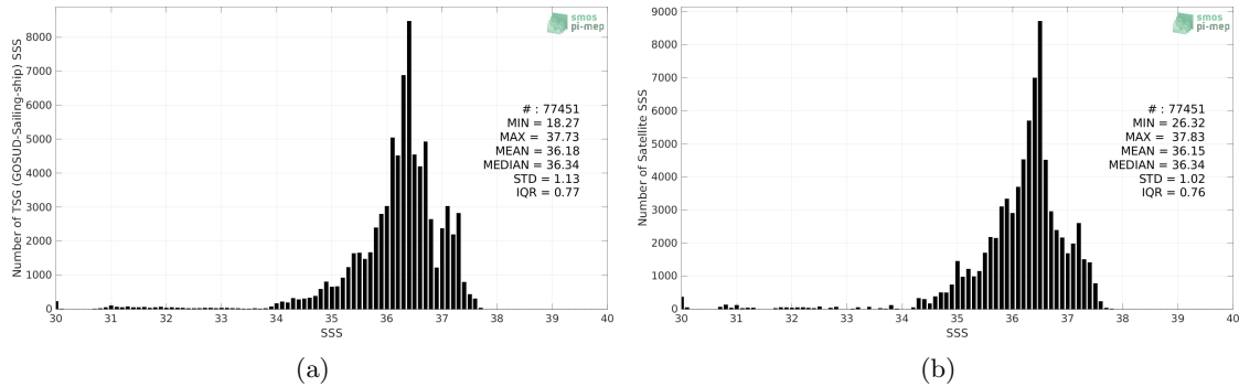
Figure 2: Histograms of SSS from TSG (GOSUD-Sailing-ship) (a) and SMOS SSS L3 v332 - 9 Days (CATDS-CPDC) (b) considering all match-up pairs per bins of 0.1 over the Tropical Atlantic Ocean Pi-MEP region and for the full satellite product period.
