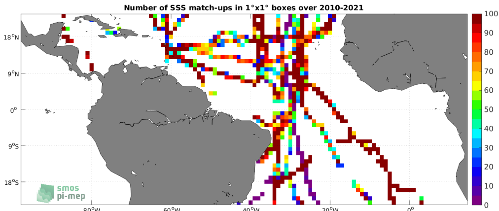
Figure 4: Number of SSS match-ups between TSG (GOSUD-Sailing-ship) SSS and the SMOS SSS L3 v332 - 9 Days (CATDS-CPDC) SSS product for the Tropical Atlantic Ocean Pi-MEP region over 1^\circ \times 1^\circ boxes and for the full satellite product period.
