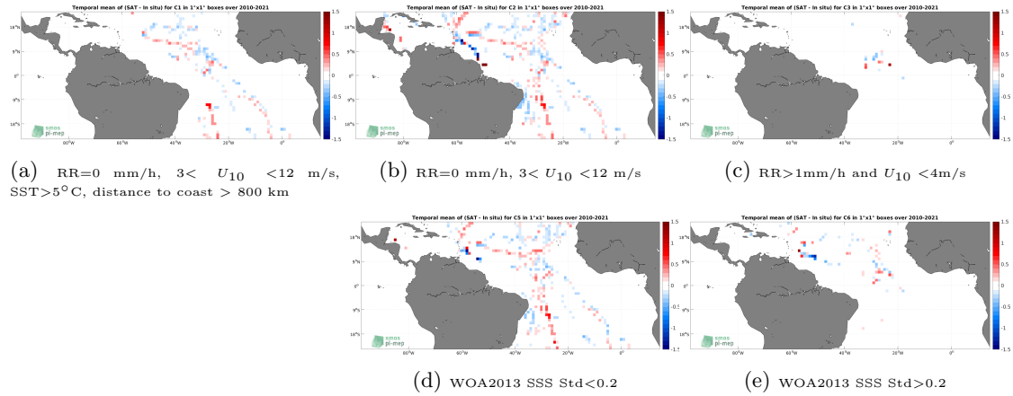
Figure 12: Temporal mean gridded over spatial boxes of size 1^{\circ}\times 1^{\circ} of \Delta SSS (SMOS SSS L3 v332 - 9 Days (CATDS-CPDC) - TSG (GOSUD-Sailing-ship)) for 5 different subdatasets corresponding to: RR=0 mm/h, 3 < U_{10} < 12 m/s, SST > 5^{\circ}\text{C} , distance to coast > 800 km (a), RR=0 mm/h, 3 < U_{10} < 12 m/s (b), RR > 1 mm/h and U_{10} < 4 m/s (c), WOA2013 SSS Std < 0.2 (d), WOA2013 SSS Std > 0.2 (e).
