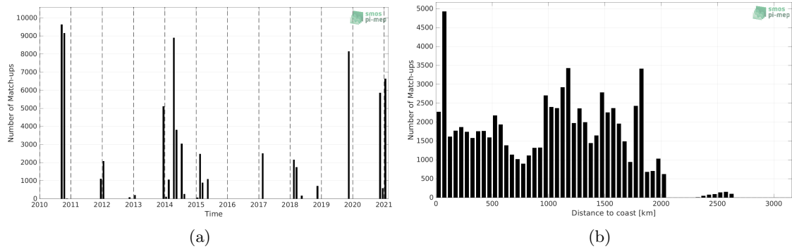
Figure 1: Number of match-ups between TSG (GOSUD-Sailing-ship) and SMOS SSS L3 v332 - 9 Days (CATDS-CPDC) SSS as a function of time (a) and as function of the distance to coast (b) over the Tropical Atlantic Ocean Pi-MEP region and for the full satellite product period.
