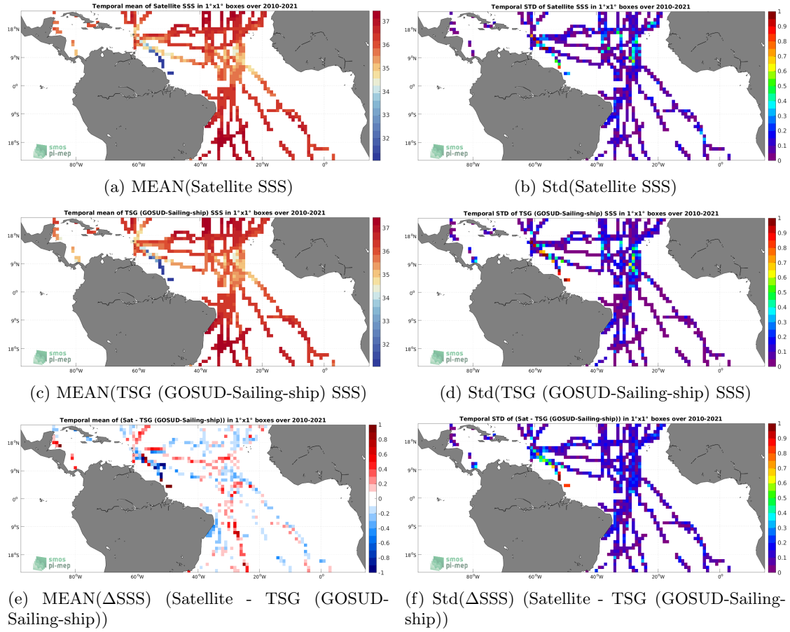
Figure 6: Temporal mean (left) and Std (right) of SSS from SMOS SSS L3 v332 - 9 Days (CATDS-CPDC) (top), TSG (GOSUD-Sailing-ship) (middle), and of \Delta SSS (Satellite - TSG (GOSUD-Sailing-ship)). Only match-up pairs are used to generate these maps.
