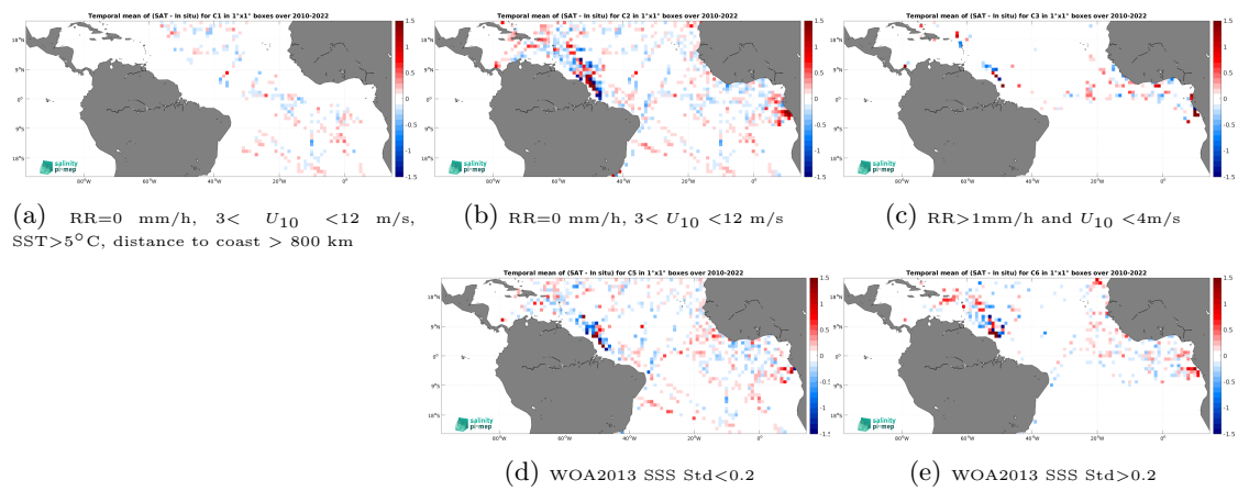
Figure 14: Temporal mean gridded over spatial boxes of size 1^\circ \times 1^\circ of \Delta\text{SSS} (SMOS SSS L3 v332 - 9 Days (CATDS-CPDC) - TSG (GOSUD-Research-vessel)) for 5 different subdatasets corresponding to:RR=0 mm/h, 3 < U_{10} < 12 m/s, SST >5^\circ\text{C} , distance to coast > 800 km (a), RR=0 mm/h, 3 < U_{10} < 12 m/s (b), RR >1 mm/h and U_{10} < 4 m/s (c), WOA2013 SSS Std <0.2 (d), WOA2013 SSS Std >0.2 (e).
