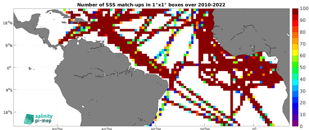
Figure 5: Number of SSS match-ups between TSG (GOSUD-Research-vessel) SSS and the SMOS SSS L3 v332 - 9 Days (CATDS-CPDC) SSS product for the Tropical Atlantic Ocean Pi-MEP region over 1^\circ \times 1^\circ boxes and for the full satellite product period.
