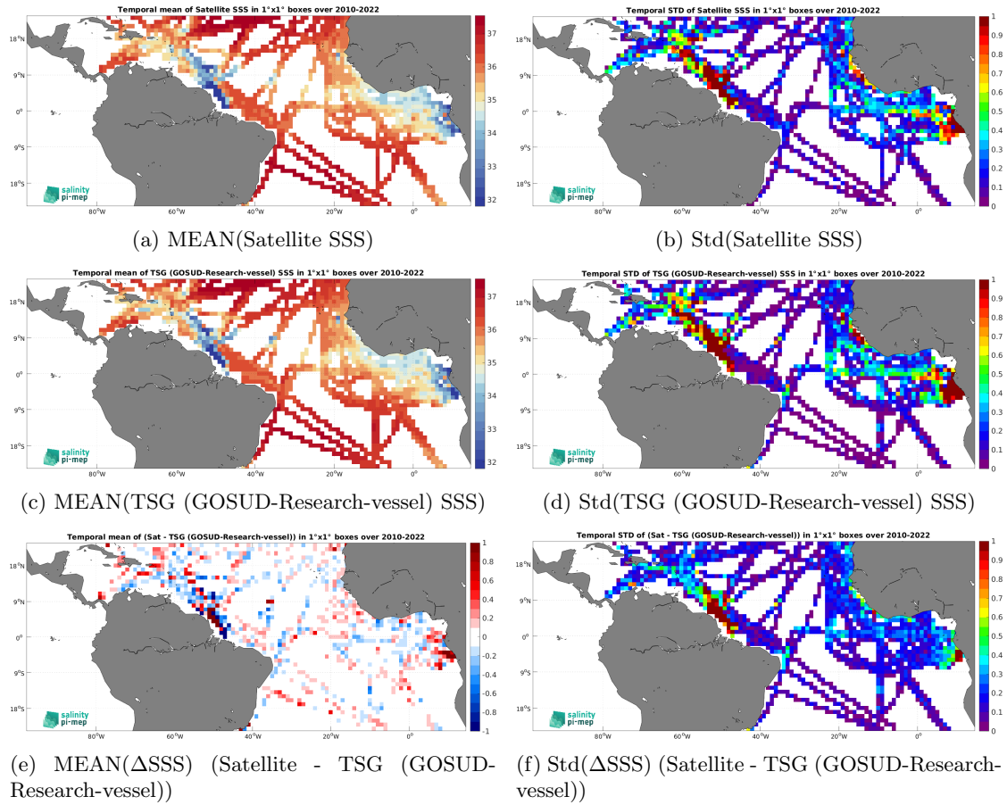
Figure 7: Temporal mean (left) and Std (right) of SSS from SMOS SSS L3 v332 - 9 Days (CATDS-CPDC) (top), TSG (GOSUD-Research-vessel) (middle), and of \Delta SSS (Satellite - TSG (GOSUD-Research-vessel)). Only match-up pairs are used to generate these maps.
