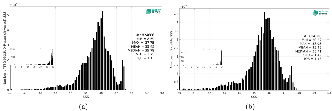
Figure 3: Histograms of SSS from TSG (GOSUD-Research-vessel) (a) and SMOS SSS L3 v332 - 9 Days (CATDS-CPDC) (b) considering all match-up pairs per bins of 0.1 over the Tropical Atlantic Ocean Pi-MEP region and for the full satellite product period.
