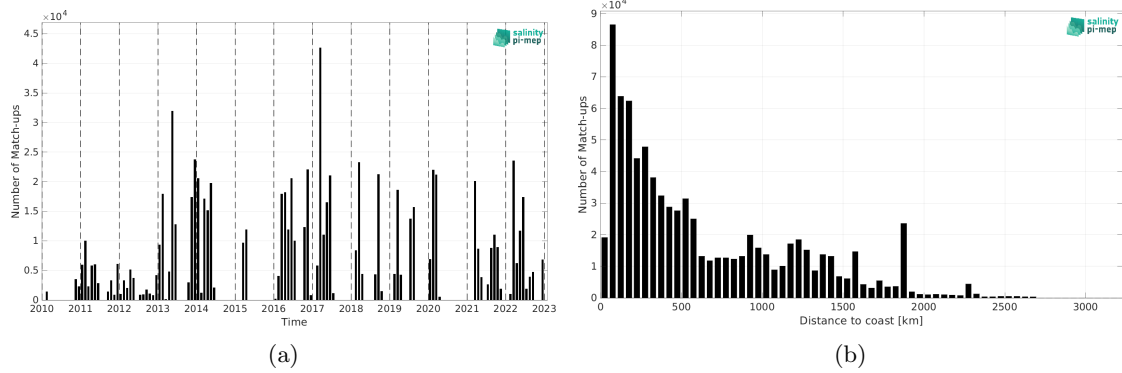
Figure 2: Number of match-ups between TSG (GOSUD-Research-vessel) and SMOS SSS L3 v332 - 9 Days (CATDS-CPDC) SSS as a function of time (a) and as function of the distance to coast (b) over the Tropical Atlantic Ocean Pi-MEP region and for the full satellite product period.
