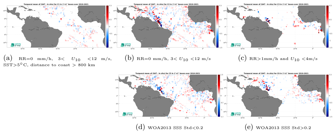
Figure 12: Temporal mean gridded over spatial boxes of size 1^\circ \times 1^\circ of \Delta\text{SSS} (SMOS SSS L3 v332 - 9 Days (CATDS-CPDC) - TSG (GOSUD-Research-vessel)) for 5 different subdatasets corresponding to:RR=0 mm/h, 3 < U_{10} < 12 m/s, SST >5^\circ\text{C} , distance to coast > 800 km (a), RR=0 mm/h, 3 < U_{10} < 12 m/s (b), RR >1 mm/h and U_{10} < 4 m/s (c), WOA2013 SSS Std <0.2 (d), WOA2013 SSS Std >0.2 (e).
