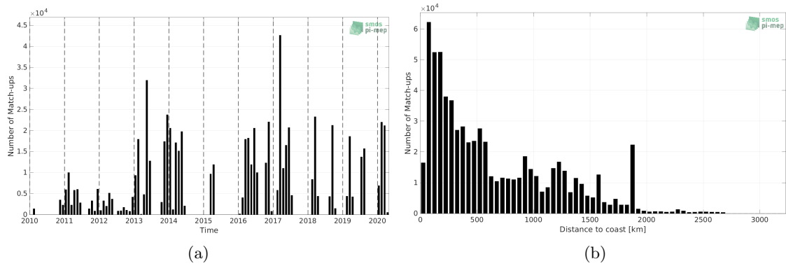
Figure 1: Number of match-ups between TSG (GOSUD-Research-vessel) and SMOS SSS L3 v332 - 9 Days (CATDS-CPDC) SSS as a function of time (a) and as function of the distance to coast (b) over the Tropical Atlantic Ocean Pi-MEP region and for the full satellite product period.
