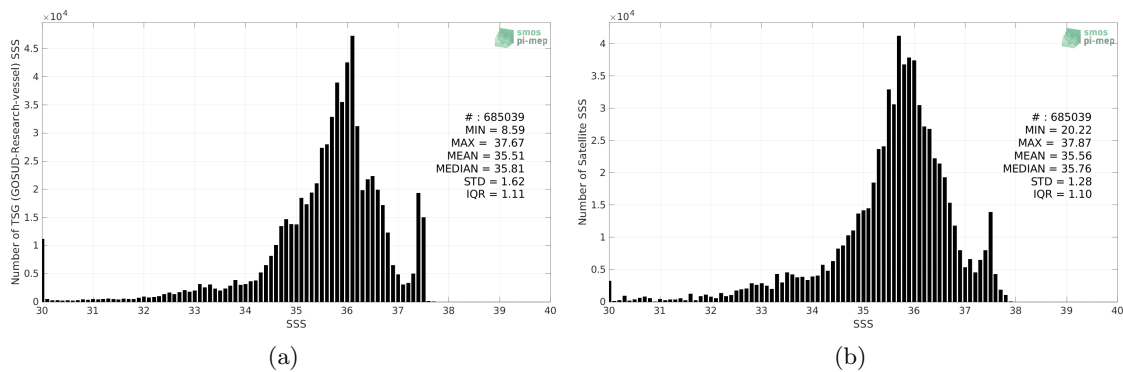
Figure 2: Histograms of SSS from TSG (GOSUD-Research-vessel) (a) and SMOS SSS L3 v332 - 9 Days (CATDS-CPDC) (b) considering all match-up pairs per bins of 0.1 over the Tropical Atlantic Ocean Pi-MEP region and for the full satellite product period.
