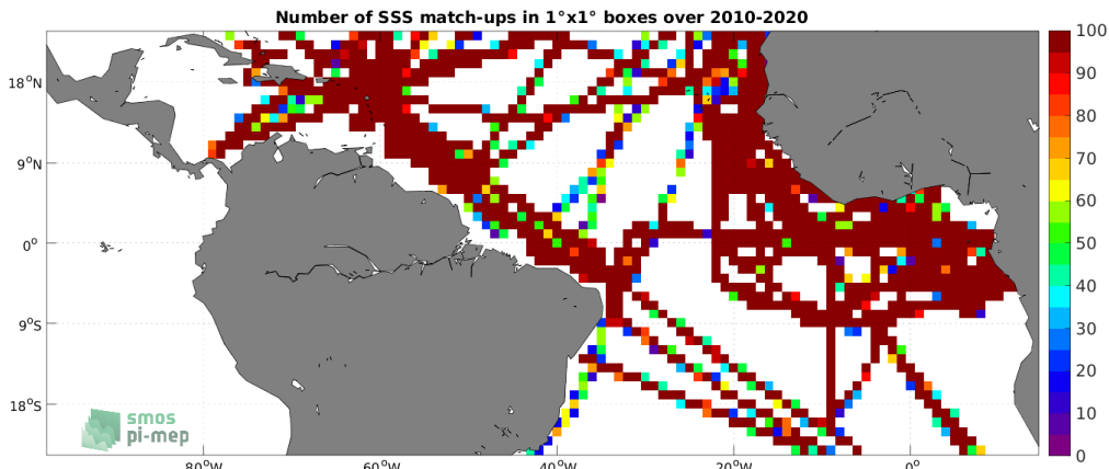
Figure 4: Number of SSS match-ups between TSG (GOSUD-Research-vessel) SSS and the SMOS SSS L3 v332 - 9 Days (CATDS-CPDC) SSS product for the Tropical Atlantic Ocean Pi-MEP region over 1^\circ \times 1^\circ boxes and for the full satellite product period.
