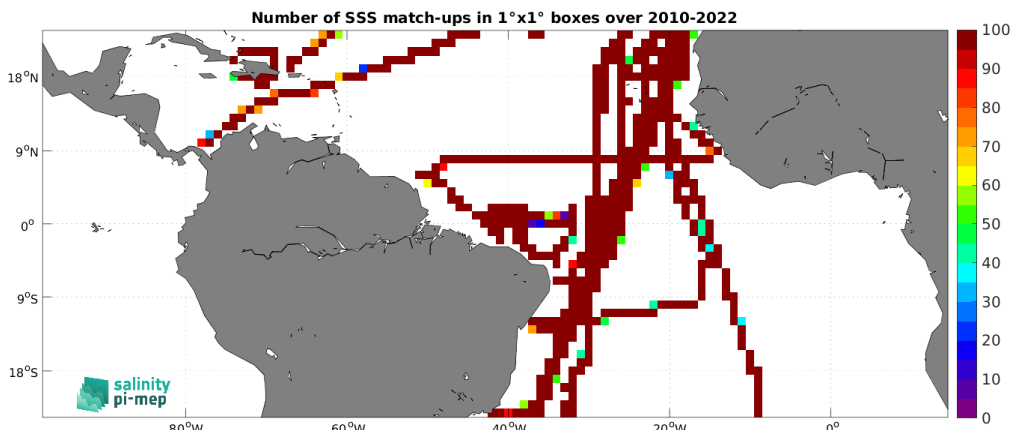
Figure 5: Number of SSS match-ups between TSG (CSIC-UTM) SSS and the SMOS SSS L3 v332 - 9 Days (CATDS-CPDC) SSS product for the Tropical Atlantic Ocean Pi-MEP region over 1^\circ \times 1^\circ boxes and for the full satellite product period.
