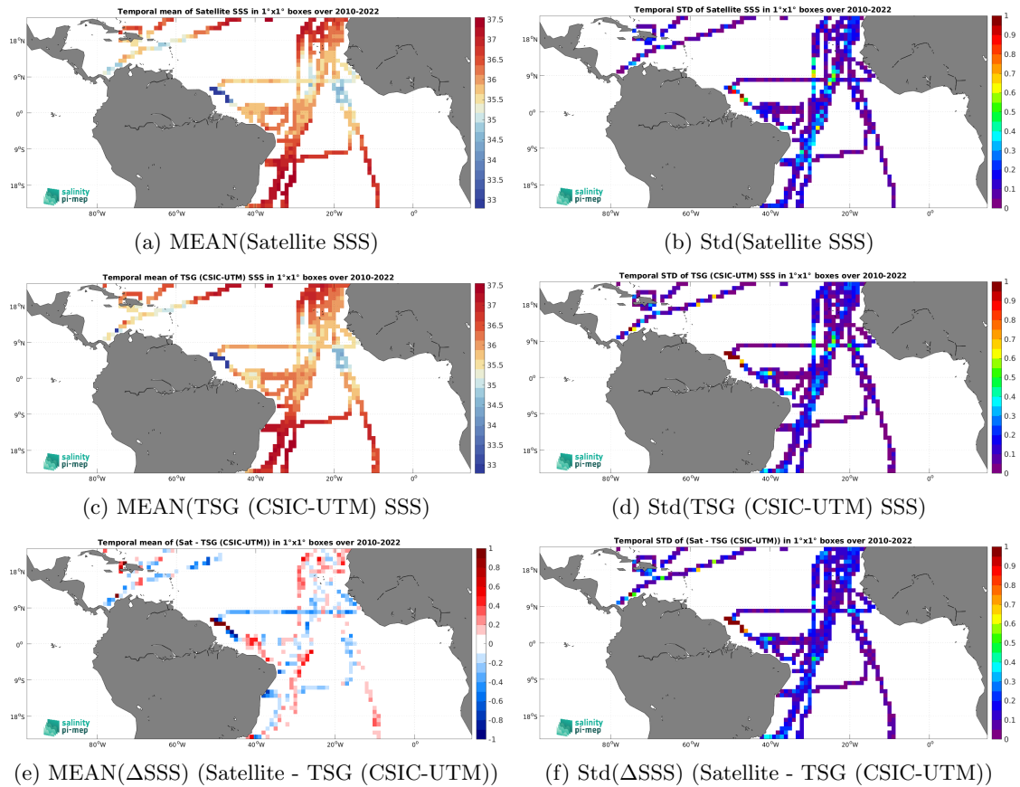
Figure 7: Temporal mean (left) and Std (right) of SSS from SMOS SSS L3 v332 - 9 Days (CATDS-CPDC) (top), TSG (CSIC-UTM) (middle), and of \Delta SSS (Satellite - TSG (CSIC-UTM)). Only match-up pairs are used to generate these maps.
