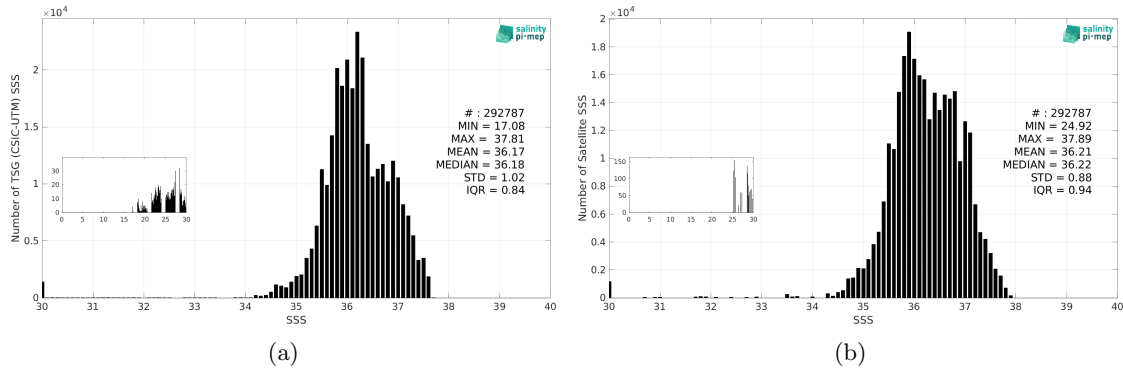
Figure 3: Histograms of SSS from TSG (CSIC-UTM) (a) and SMOS SSS L3 v332 - 9 Days (CATDS-CPDC) (b) considering all match-up pairs per bins of 0.1 over the Tropical Atlantic Ocean Pi-MEP region and for the full satellite product period.
