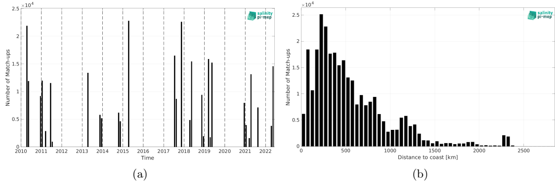
Figure 2: Number of match-ups between TSG (CSIC-UTM) and SMOS SSS L3 v332 - 9 Days (CATDS-CPDC) SSS as a function of time (a) and as function of the distance to coast (b) over the Tropical Atlantic Ocean Pi-MEP region and for the full satellite product period.
