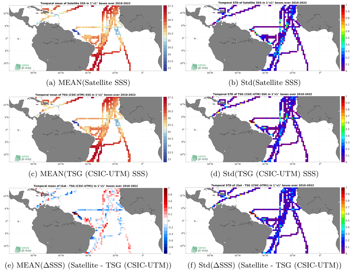
Figure 6: Temporal mean (left) and Std (right) of SSS from SMOS SSS L3 v332 - 9 Days (CATDS-CPDC) (top), TSG (CSIC-UTM) (middle), and of \Delta SSS (Satellite - TSG (CSIC-UTM)). Only match-up pairs are used to generate these maps.
