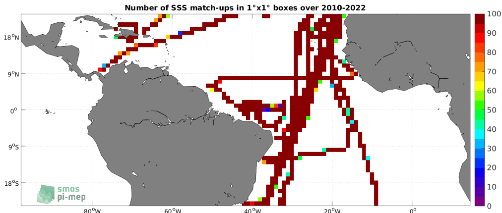
Figure 4: Number of SSS match-ups between TSG (CSIC-UTM) SSS and the SMOS SSS L3 v332 - 9 Days (CATDS-CPDC) SSS product for the Tropical Atlantic Ocean Pi-MEP region over 1^\circ \times 1^\circ boxes and for the full satellite product period.
