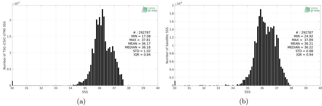
Figure 2: Histograms of SSS from TSG (CSIC-UTM) (a) and SMOS SSS L3 v332 - 9 Days (CATDS-CPDC) (b) considering all match-up pairs per bins of 0.1 over the Tropical Atlantic Ocean Pi-MEP region and for the full satellite product period.
