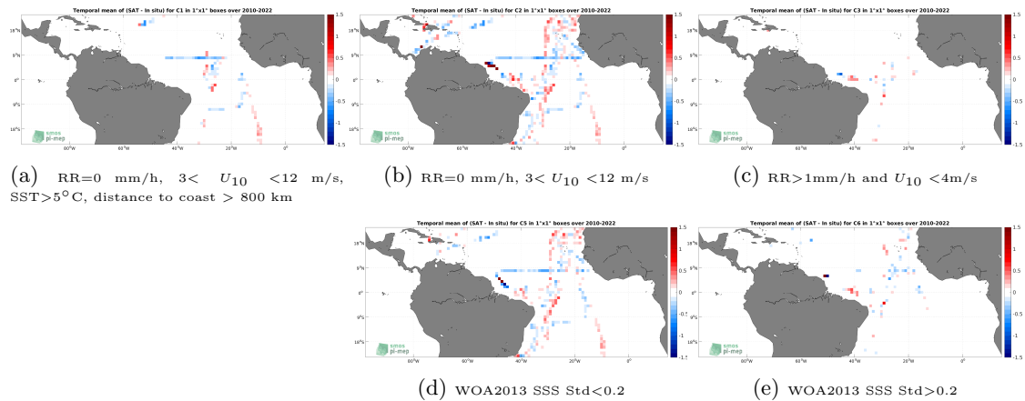
Figure 12: Temporal mean gridded over spatial boxes of size 1^\circ \times 1^\circ of \Delta SSS (SMOS SSS L3 v332 - 9 Days (CATDS-CPDC) - TSG (CSIC-UTM)) for 5 different subdatasets corresponding to:RR=0 mm/h, 3 < U_{10} < 12 m/s, SST >5^\circ\text{C} , distance to coast > 800 km (a), RR=0 mm/h, 3 < U_{10} < 12 m/s (b), RR >1 mm/h and U_{10} < 4 m/s (c), WOA2013 SSS Std <0.2 (d), WOA2013 SSS Std >0.2 (e).
