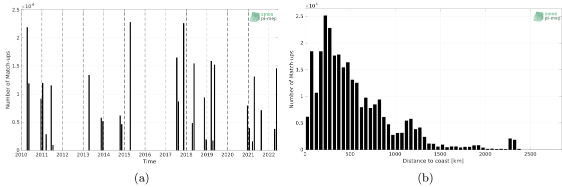
Figure 1: Number of match-ups between TSG (CSIC-UTM) and SMOS SSS L3 v332 - 9 Days (CATDS-CPDC) SSS as a function of time (a) and as function of the distance to coast (b) over the Tropical Atlantic Ocean Pi-MEP region and for the full satellite product period.
