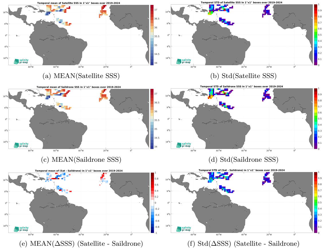
Figure 7: Temporal mean (left) and Std (right) of SSS from SMOS SSS L3 v332 - 9 Days (CATDS-CPDC) (top), Saildrone (middle), and of \Delta SSS (Satellite - Saildrone). Only match-up pairs are used to generate these maps.
