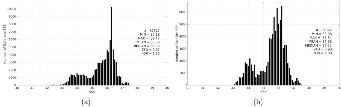
Figure 3: Histograms of SSS from Saildrone (a) and SMOS SSS L3 v332 - 9 Days (CATDS-CPDC) (b) considering all match-up pairs per bins of 0.1 over the Tropical Atlantic Ocean Pi-MEP region and for the full satellite product period.
