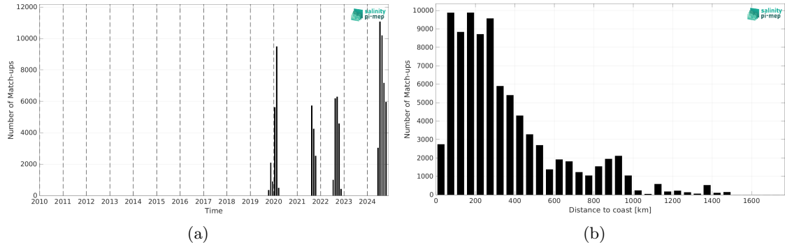
Figure 2: Number of match-ups between Saildrone and SMOS SSS L3 v332 - 9 Days (CATDS-CPDC) SSS as a function of time (a) and as function of the distance to coast (b) over the Tropical Atlantic Ocean Pi-MEP region and for the full satellite product period.
