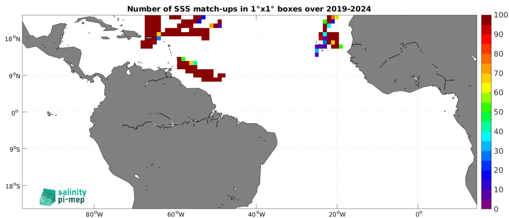
Figure 5: Number of SSS match-ups between Saildrone SSS and the SMOS SSS L3 v332 - 9 Days (CATDS-CPDC) SSS product for the Tropical Atlantic Ocean Pi-MEP region over 1^\circ \times 1^\circ boxes and for the full satellite product period.
