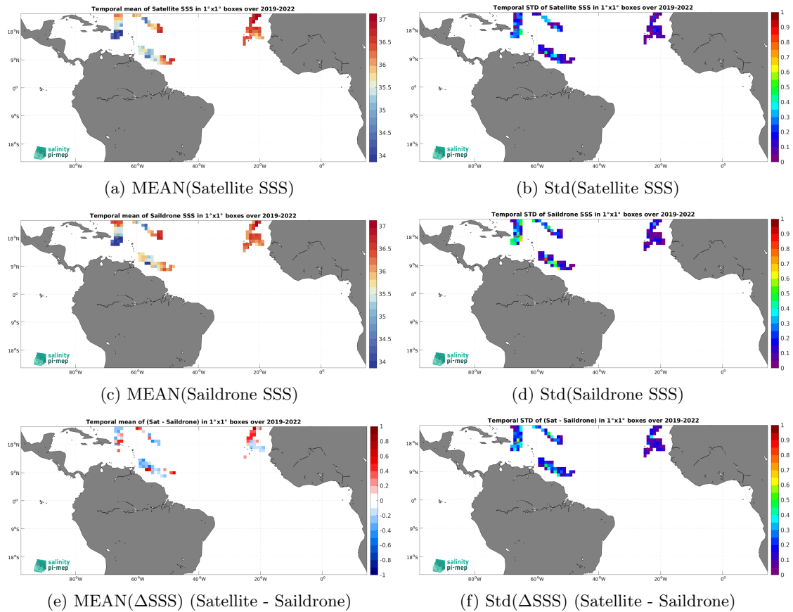
Figure 6: Temporal mean (left) and Std (right) of SSS from SMOS SSS L3 v332 - 9 Days (CATDS-CPDC) (top), Saildrone (middle), and of \Delta SSS (Satellite - Saildrone). Only match-up pairs are used to generate these maps.
