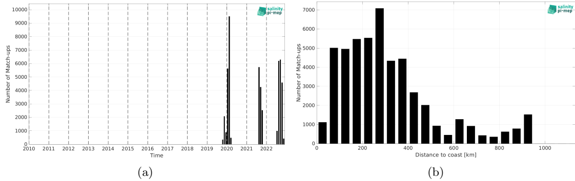
Figure 1: Number of match-ups between Saildrone and SMOS SSS L3 v332 - 9 Days (CATDS-CPDC) SSS as a function of time (a) and as function of the distance to coast (b) over the Tropical Atlantic Ocean Pi-MEP region and for the full satellite product period.
