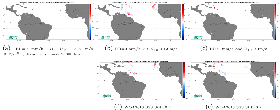
Figure 12: Temporal mean gridded over spatial boxes of size 1^\circ \times 1^\circ of \Delta\text{SSS} (SMOS SSS L3 v332 - 9 Days (CATDS-CPDC) - Sairdrone) for 5 different subdatasets corresponding to:RR=0 mm/h, 3 < U_{10} < 12 m/s, SST >5^\circ\text{C} , distance to coast > 800 km (a), RR=0 mm/h, 3 < U_{10} < 12 m/s (b), RR >1 mm/h and U_{10} < 4 m/s (c), WOA2013 SSS Std <0.2 (d), WOA2013 SSS Std >0.2 (e).
