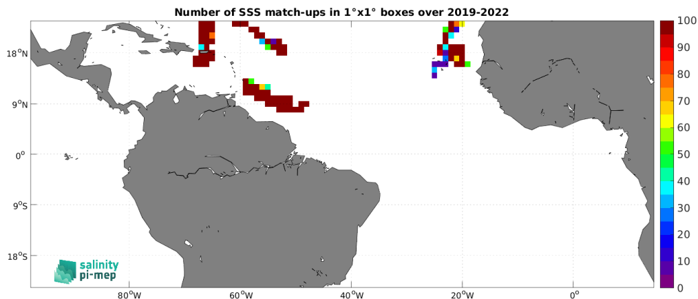
Figure 4: Number of SSS match-ups between Saildrone SSS and the SMOS SSS L3 v332 - 9 Days (CATDS-CPDC) SSS product for the Tropical Atlantic Ocean Pi-MEP region over 1^\circ \times 1^\circ boxes and for the full satellite product period.
