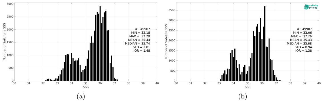
Figure 2: Histograms of SSS from Saildrone (a) and SMOS SSS L3 v332 - 9 Days (CATDS-CPDC) (b) considering all match-up pairs per bins of 0.1 over the Tropical Atlantic Ocean Pi-MEP region and for the full satellite product period.
