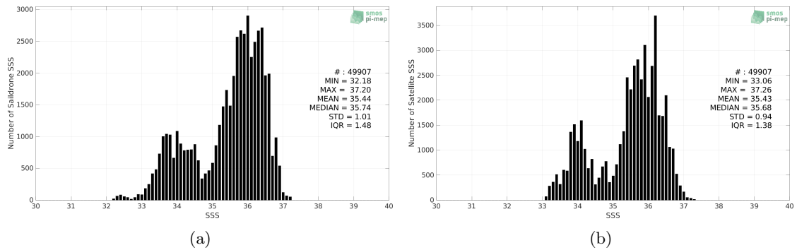
Figure 2: Histograms of SSS from Sairdrone (a) and SMOS SSS L3 v332 - 9 Days (CATDS-CPDC) (b) considering all match-up pairs per bins of 0.1 over the Tropical Atlantic Ocean Pi-MEP region and for the full satellite product period.
