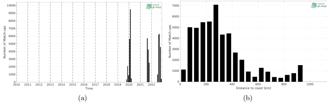
Figure 1: Number of match-ups between Sairdrone and SMOS SSS L3 v332 - 9 Days (CATDS-CPDC) SSS as a function of time (a) and as function of the distance to coast (b) over the Tropical Atlantic Ocean Pi-MEP region and for the full satellite product period.
