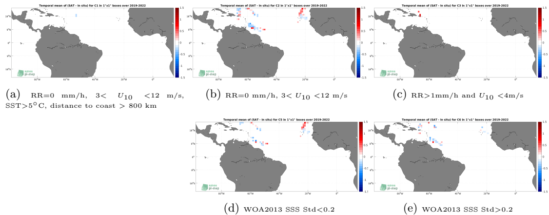
Figure 12: Temporal mean gridded over spatial boxes of size 1^\circ \times 1^\circ of \Delta SSS (SMOS SSS L3 v332 - 9 Days (CATDS-CPDC) - Sairdrone) for 5 different subdatasets corresponding to:RR=0 mm/h, 3 < U_{10} < 12 m/s, SST >5^\circ\text{C} , distance to coast > 800 km (a), RR=0 mm/h, 3 < U_{10} < 12 m/s (b), RR >1 mm/h and U_{10} < 4 m/s (c), WOA2013 SSS Std <0.2 (d), WOA2013 SSS Std >0.2 (e).
