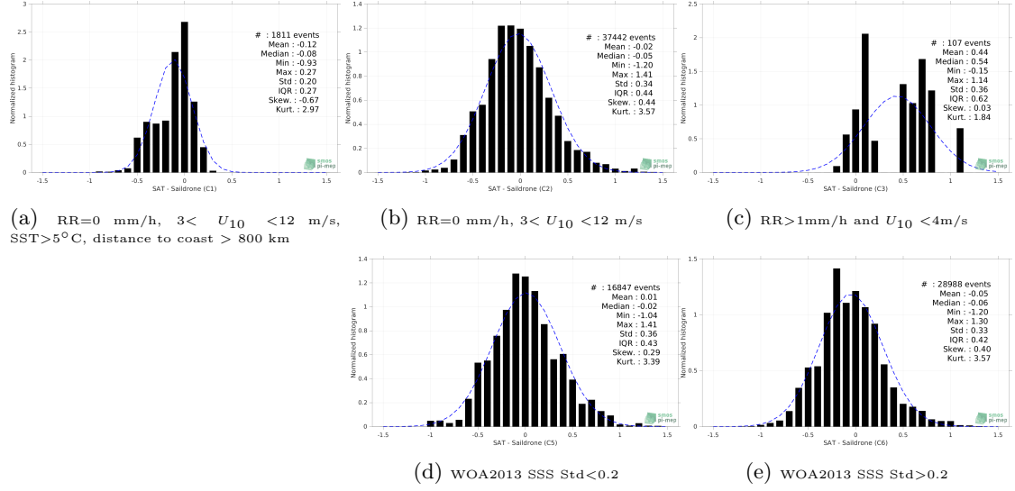
Figure 13: Normalized histogram of \Delta SSS (SMOS SSS L3 v332 - 9 Days (CATDS-CPDC) - Saildrone) for 5 different subdatasets corresponding to: RR=0 mm/h, 3 < U_{10} < 12 m/s, SST>5°C, distance to coast > 800 km (a), RR=0 mm/h, 3 < U_{10} < 12 m/s (b), RR>1mm/h and U_{10} < 4 m/s (c), WOA2013 SSS Std<0.2 (d), WOA2013 SSS Std>0.2 (e).
