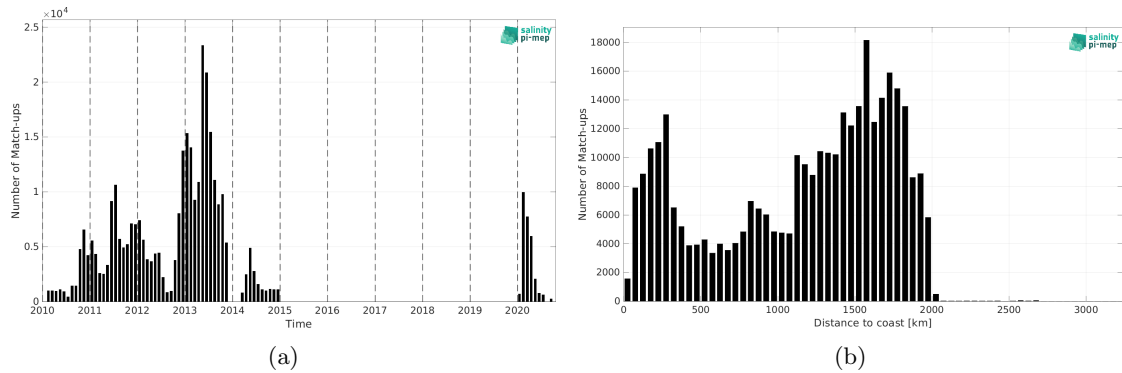
Figure 2: Number of match-ups between Surface drifters and SMOS SSS L3 v332 - 9 Days (CATDS-CPDC) SSS as a function of time (a) and as function of the distance to coast (b) over the Tropical Atlantic Ocean Pi-MEP region and for the full satellite product period.
