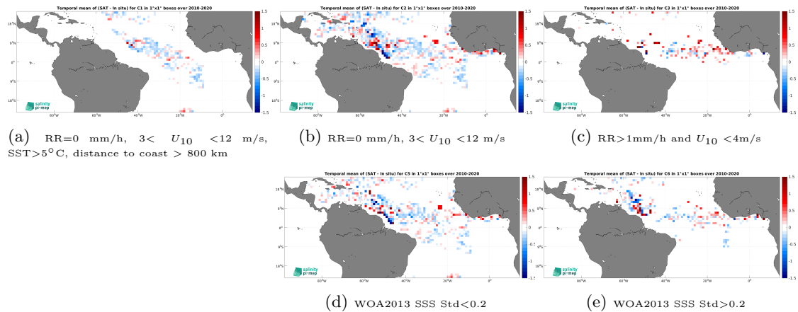
Figure 13: Temporal mean gridded over spatial boxes of size 1^\circ \times 1^\circ of \Delta\text{SSS} (SMOS SSS L3 v332 - 9 Days (CATDS-CPDC) - Surface drifters) for 5 different subdatasets corresponding to:RR=0 mm/h, 3 < U_{10} < 12 m/s, SST >5^\circ\text{C} , distance to coast > 800 km (a), RR=0 mm/h, 3 < U_{10} < 12 m/s (b), RR >1 mm/h and U_{10} < 4 m/s (c), WOA2013 SSS Std <0.2 (d), WOA2013 SSS Std >0.2 (e).
