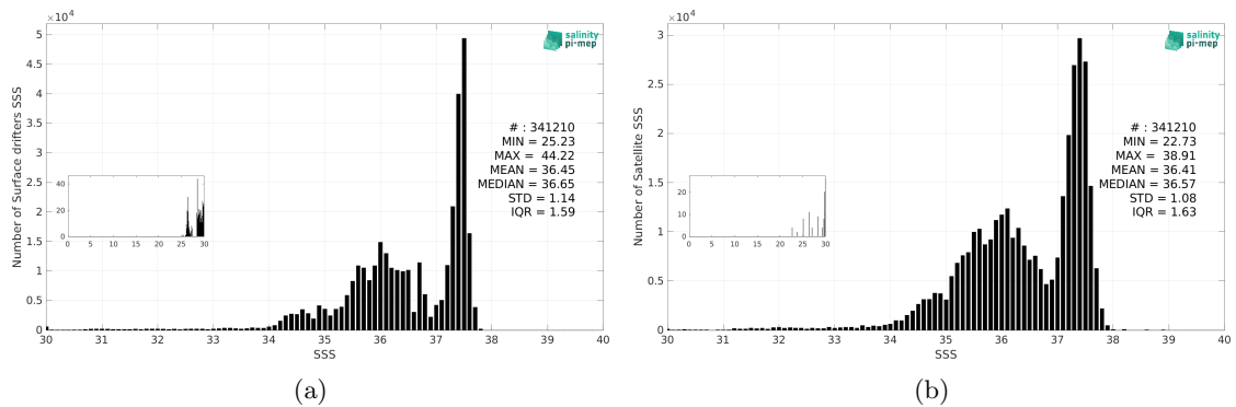
Figure 3: Histograms of SSS from Surface drifters (a) and SMOS SSS L3 v332 - 9 Days (CATDS-CPDC) (b) considering all match-up pairs per bins of 0.1 over the Tropical Atlantic Ocean Pi-MEP region and for the full satellite product period.
