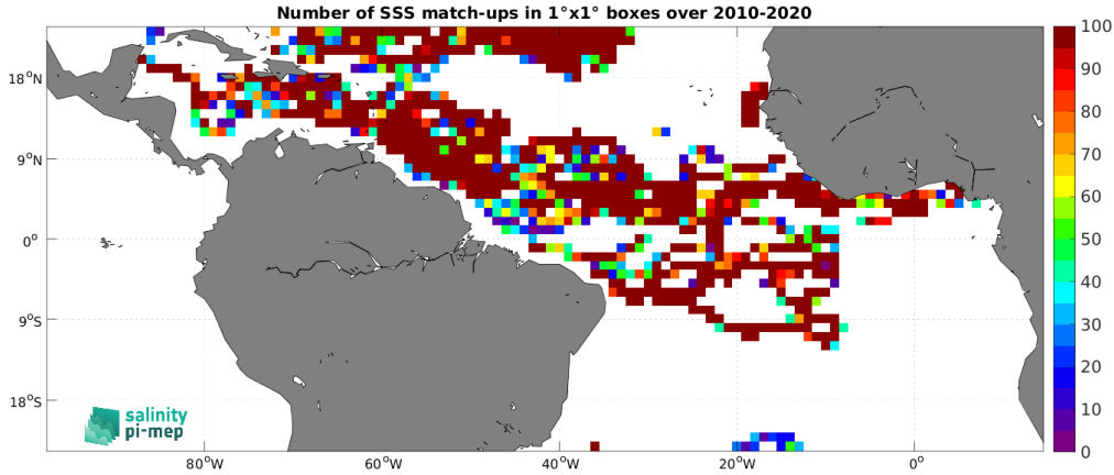
Figure 4: Number of SSS match-ups between Surface drifters SSS and the SMOS SSS L3 v332 - 9 Days (CATDS-CPDC) SSS product for the Tropical Atlantic Ocean Pi-MEP region over 1^\circ \times 1^\circ boxes and for the full satellite product period.
