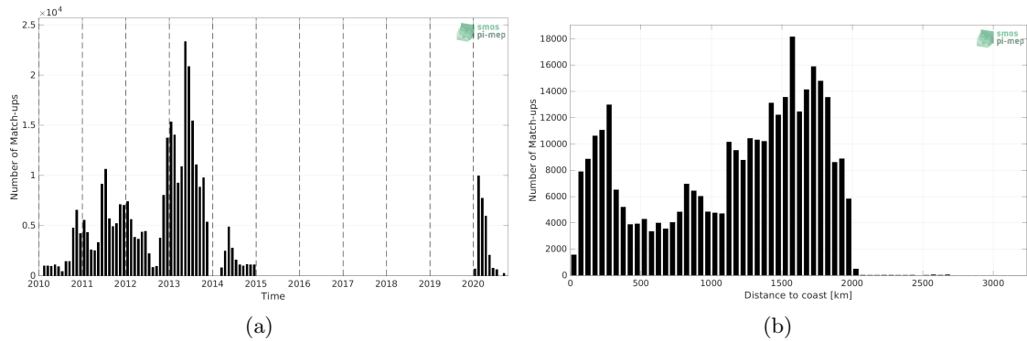
Figure 1: Number of match-ups between Surface drifters and SMOS SSS L3 v332 - 9 Days (CATDS-CPDC) SSS as a function of time (a) and as function of the distance to coast (b) over the Tropical Atlantic Ocean Pi-MEP region and for the full satellite product period.
