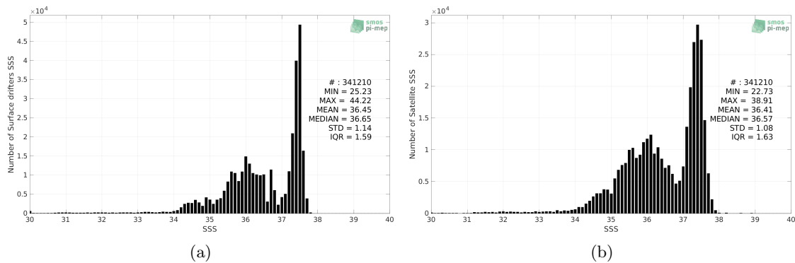
Figure 2: Histograms of SSS from Surface drifters (a) and SMOS SSS L3 v332 - 9 Days (CATDS-CPDC) (b) considering all match-up pairs per bins of 0.1 over the Tropical Atlantic Ocean Pi-MEP region and for the full satellite product period.
