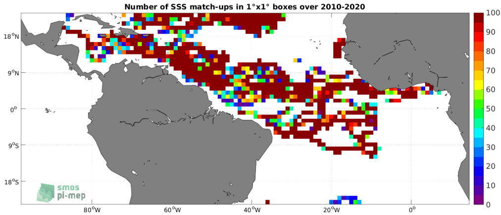
Figure 3: Number of SSS match-ups between Surface drifters SSS and the SMOS SSS L3 v332 - 9 Days (CATDS-CPDC) SSS product for the Tropical Atlantic Ocean Pi-MEP region over 1^\circ \times 1^\circ boxes and for the full satellite product period.
