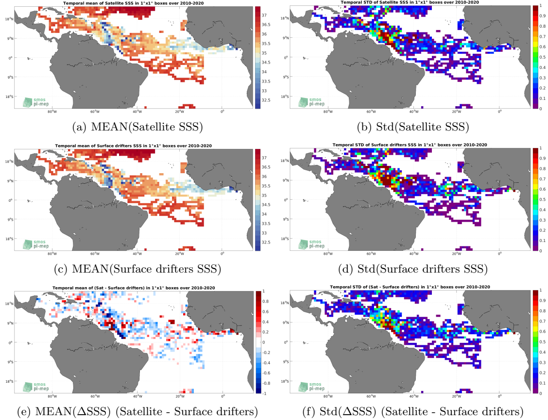
Figure 5: Temporal mean (left) and Std (right) of SSS from SMOS SSS L3 v332 - 9 Days (CATDS-CPDC) (top), Surface drifters (middle), and of \Delta SSS (Satellite - Surface drifters). Only match-up pairs are used to generate these maps.
