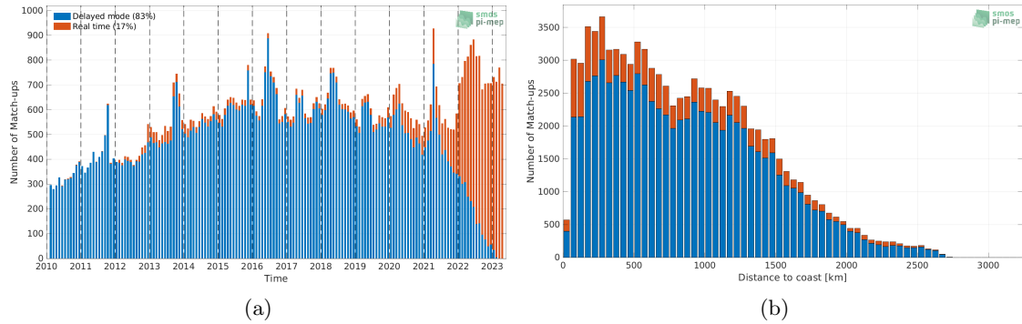
Figure 1: Number of match-ups between Argo and SMOS SSS L3 v332 - 9 Days (CATDS-CPDC) SSS as a function of time (a) and as function of the distance to coast (b) over the Tropical Atlantic Ocean Pi-MEP region and for the full satellite product period.
