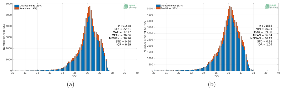
Figure 2: Histograms of SSS from Argo (a) and SMOS SSS L3 v332 - 9 Days (CATDS-CPDC) (b) considering all match-up pairs per bins of 0.1 over the Tropical Atlantic Ocean Pi-MEP region and for the full satellite product period.
