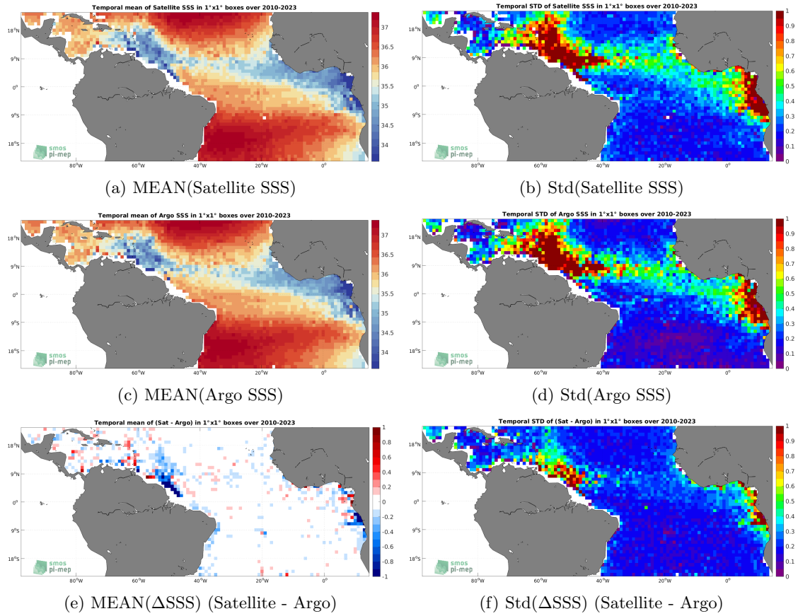
Figure 6: Temporal mean (left) and Std (right) of SSS from SMOS SSS L3 v332 - 9 Days (CATDS-CPDC) (top), Argo (middle), and of \Delta SSS (Satellite - Argo). Only match-up pairs are used to generate these maps.
