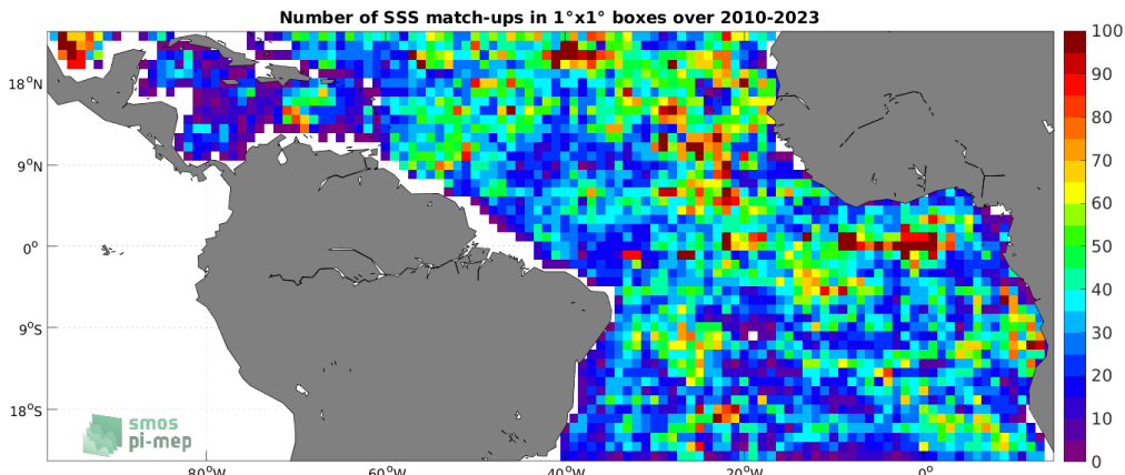
Figure 4: Number of SSS match-ups between Argo SSS and the SMOS SSS L3 v332 - 9 Days (CATDS-CPDC) SSS product for the Tropical Atlantic Ocean Pi-MEP region over 1^\circ \times 1^\circ boxes and for the full satellite product period.
