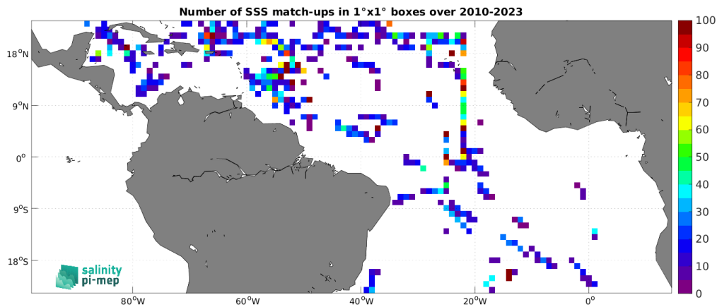
Figure 4: Number of SSS match-ups between TSG (SAMOS) SSS and the SMOS SSS L2Q v331 - 0.25 Deg (CATDS-CPDC) SSS product for the Tropical Atlantic Ocean Pi-MEP region over 1^\circ \times 1^\circ boxes and for the full satellite product period.
