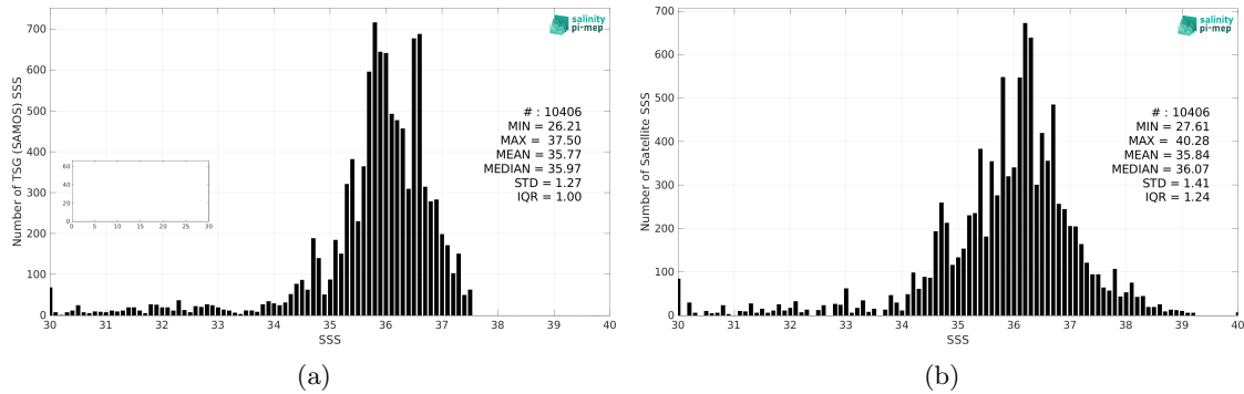
Figure 2: Histograms of SSS from TSG (SAMOS) (a) and SMOS SSS L2Q v331 - 0.25 Deg (CATDS-CPDC) (b) considering all match-up pairs per bins of 0.1 over the Tropical Atlantic Ocean Pi-MEP region and for the full satellite product period.
