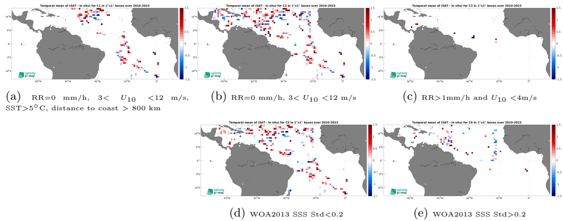
Figure 12: Temporal mean gridded over spatial boxes of size 1^\circ \times 1^\circ of \Delta SSS (SMOS SSS L2Q v331 - 0.25 Deg (CATDS-CPDC) - TSG (SAMOS)) for 5 different subdatasets corresponding to:RR=0 mm/h, 3 < U_{10} < 12 m/s, SST >5^\circ\text{C} , distance to coast > 800 km (a), RR=0 mm/h, 3 < U_{10} < 12 m/s (b), RR >1 mm/h and U_{10} < 4 m/s (c), WOA2013 SSS Std <0.2 (d), WOA2013 SSS Std >0.2 (e).
