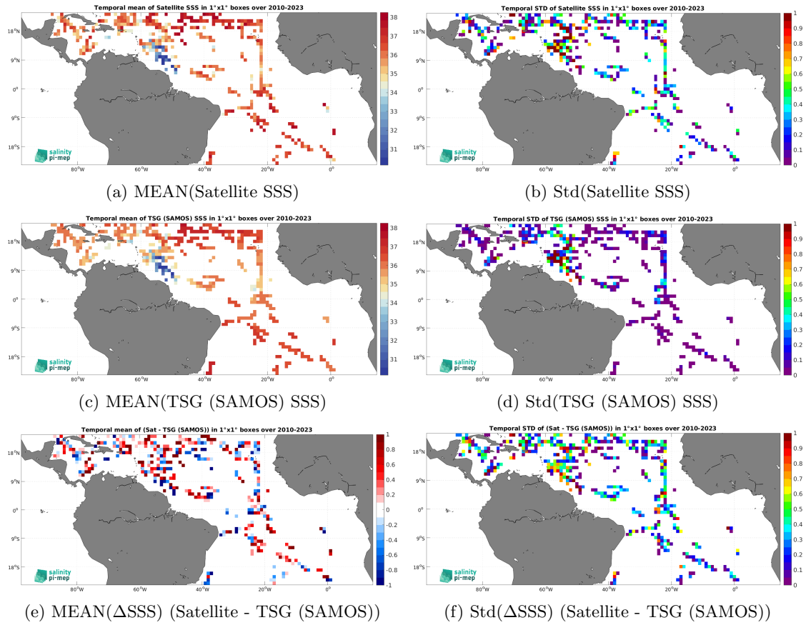
Figure 6: Temporal mean (left) and Std (right) of SSS from SMOS SSS L2Q v331 - 0.25 Deg (CATDS-CPDC) (top), TSG (SAMOS) (middle), and of \Delta SSS (Satellite - TSG (SAMOS)). Only match-up pairs are used to generate these maps.
