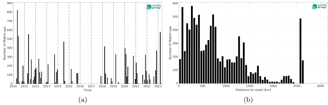
Figure 1: Number of match-ups between TSG (SAMOS) and SMOS SSS L2Q v331 - 0.25 Deg (CATDS-CPDC) SSS as a function of time (a) and as function of the distance to coast (b) over the Tropical Atlantic Ocean Pi-MEP region and for the full satellite product period.
