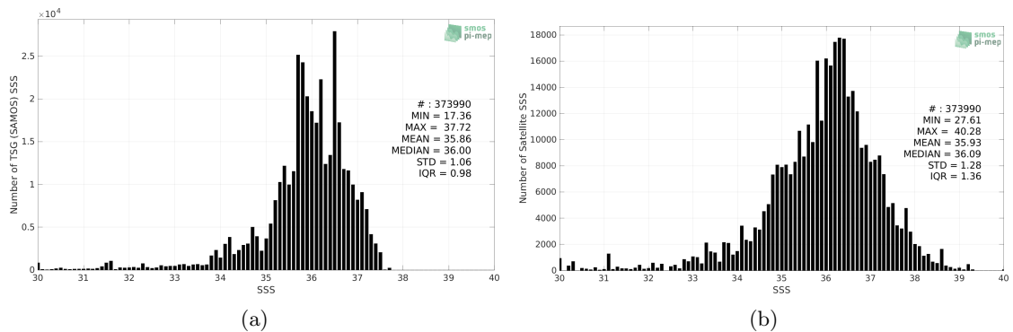
Figure 2: Histograms of SSS from TSG (SAMOS) (a) and SMOS SSS L2Q v331 - 0.25 Deg (CATDS-CPDC) (b) considering all match-up pairs per bins of 0.1 over the Tropical Atlantic Ocean Pi-MEP region and for the full satellite product period.
