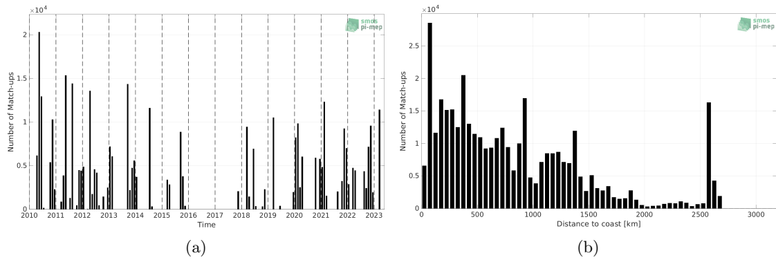
Figure 1: Number of match-ups between TSG (SAMOS) and SMOS SSS L2Q v331 - 0.25 Deg (CATDS-CPDC) SSS as a function of time (a) and as function of the distance to coast (b) over the Tropical Atlantic Ocean Pi-MEP region and for the full satellite product period.
