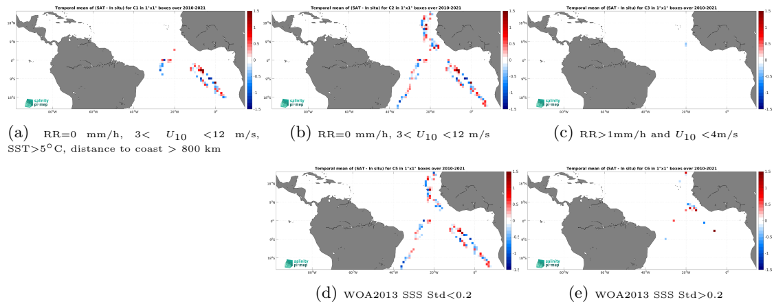
Figure 12: Temporal mean gridded over spatial boxes of size 1^\circ \times 1^\circ of \Delta\text{SSS} (SMOS SSS L2Q v331 - 0.25 Deg (CATDS-CPDC) - TSG (Polarstern)) for 5 different subdatasets corresponding to:RR=0 mm/h, 3 < U_{10} < 12 m/s, SST >5^\circ\text{C} , distance to coast > 800 km (a), RR=0 mm/h, 3 < U_{10} < 12 m/s (b), RR >1 mm/h and U_{10} < 4 m/s (c), WOA2013 SSS Std <0.2 (d), WOA2013 SSS Std >0.2 (e).
