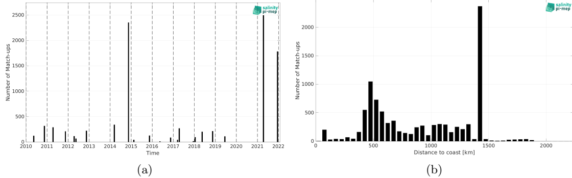
Figure 1: Number of match-ups between TSG (Polarstern) and SMOS SSS L2Q v331 - 0.25 Deg (CATDS-CPDC) SSS as a function of time (a) and as function of the distance to coast (b) over the Tropical Atlantic Ocean Pi-MEP region and for the full satellite product period.
