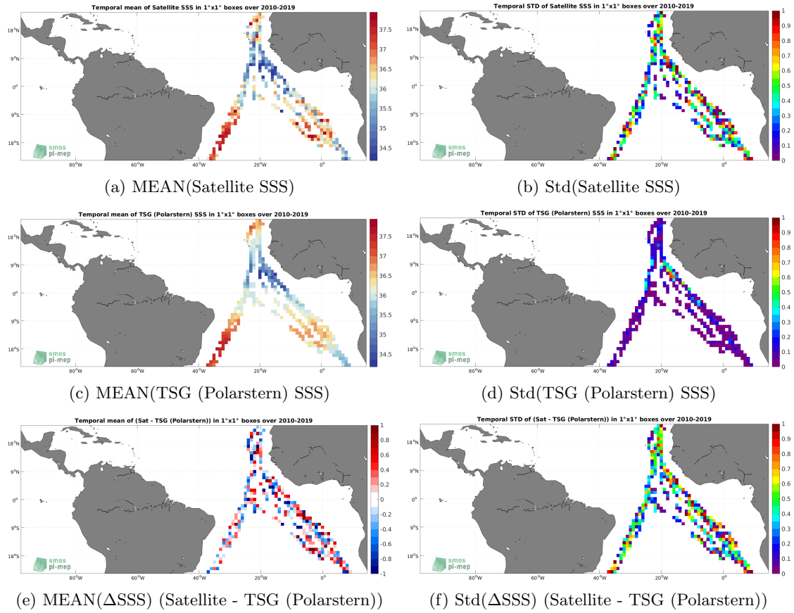
Figure 6: Temporal mean (left) and Std (right) of SSS from SMOS SSS L2Q v331 - 0.25 Deg (CATDS-CPDC) (top), TSG (Polarstern) (middle), and of \Delta SSS (Satellite - TSG (Polarstern)). Only match-up pairs are used to generate these maps.
