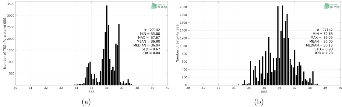
Figure 2: Histograms of SSS from TSG (Polarstern) (a) and SMOS SSS L2Q v331 - 0.25 Deg (CATDS-CPDC) (b) considering all match-up pairs per bins of 0.1 over the Tropical Atlantic Ocean Pi-MEP region and for the full satellite product period.
