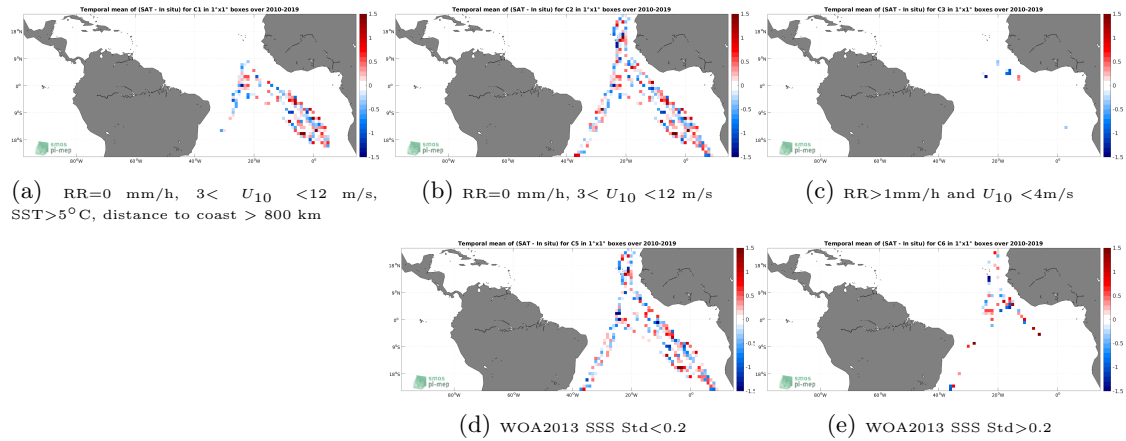
Figure 12: Temporal mean gridded over spatial boxes of size 1^\circ \times 1^\circ of \Delta SSS (SMOS SSS L2Q v331 - 0.25 Deg (CATDS-CPDC) - TSG (Polarstern)) for 5 different subdatasets corresponding to:RR=0 mm/h, 3 < U_{10} < 12 m/s, SST >5^\circ C, distance to coast > 800 km (a), RR=0 mm/h, 3 < U_{10} < 12 m/s (b), RR >1 mm/h and U_{10} < 4 m/s (c), WOA2013 SSS Std <0.2 (d), WOA2013 SSS Std >0.2 (e).
