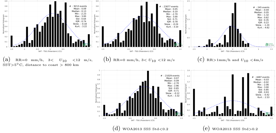
Figure 13: Normalized histogram of \Delta SSS (SMOS SSS L2Q v331 - 0.25 Deg (CATDS-CPDC) - TSG (Polarstern)) for 5 different subdatasets corresponding to: RR=0 mm/h, 3 < U_{10} < 12 m/s, SST > 5°C, distance to coast > 800 km (a), RR=0 mm/h, 3 < U_{10} < 12 m/s (b), RR > 1mm/h and U_{10} < 4 m/s (c), WOA2013 SSS Std < 0.2 (d), WOA2013 SSS Std > 0.2 (e).
