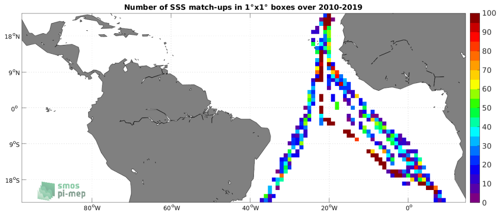
Figure 4: Number of SSS match-ups between TSG (Polarstern) SSS and the SMOS SSS L2Q v331 - 0.25 Deg (CATDS-CPDC) SSS product for the Tropical Atlantic Ocean Pi-MEP region over 1^\circ \times 1^\circ boxes and for the full satellite product period.
