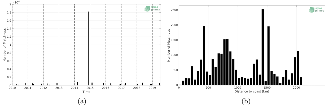
Figure 1: Number of match-ups between TSG (Polarstern) and SMOS SSS L2Q v331 - 0.25 Deg (CATDS-CPDC) SSS as a function of time (a) and as function of the distance to coast (b) over the Tropical Atlantic Ocean Pi-MEP region and for the full satellite product period.
