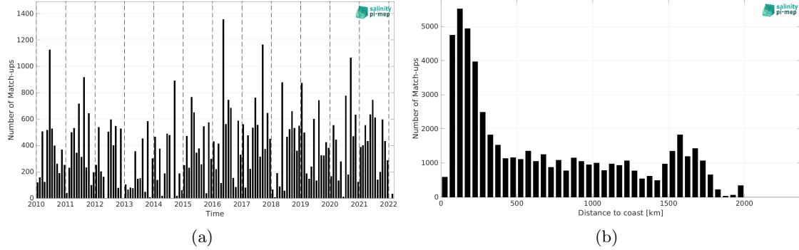
Figure 1: Number of match-ups between TSG (LEGOS-DM) and SMOS SSS L2Q v331 - 0.25 Deg (CATDS-CPDC) SSS as a function of time (a) and as function of the distance to coast (b) over the Tropical Atlantic Ocean Pi-MEP region and for the full satellite product period.
