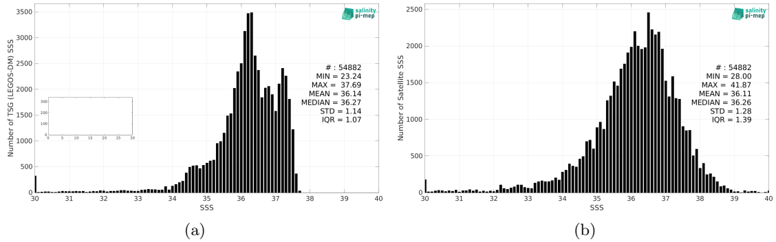
Figure 2: Histograms of SSS from TSG (LEGOS-DM) (a) and SMOS SSS L2Q v331 - 0.25 Deg (CATDS-CPDC) (b) considering all match-up pairs per bins of 0.1 over the Tropical Atlantic Ocean Pi-MEP region and for the full satellite product period.
