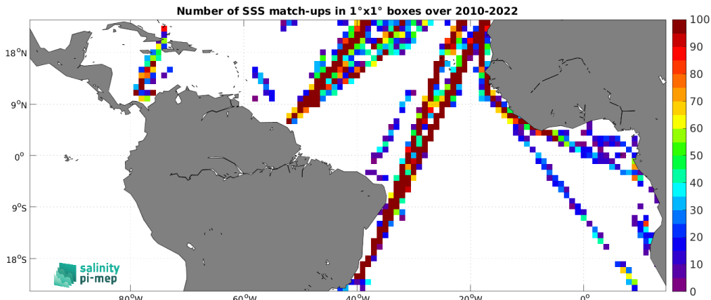
Figure 4: Number of SSS match-ups between TSG (LEGOS-DM) SSS and the SMOS SSS L2Q v331 - 0.25 Deg (CATDS-CPDC) SSS product for the Tropical Atlantic Ocean Pi-MEP region over 1^\circ \times 1^\circ boxes and for the full satellite product period.
