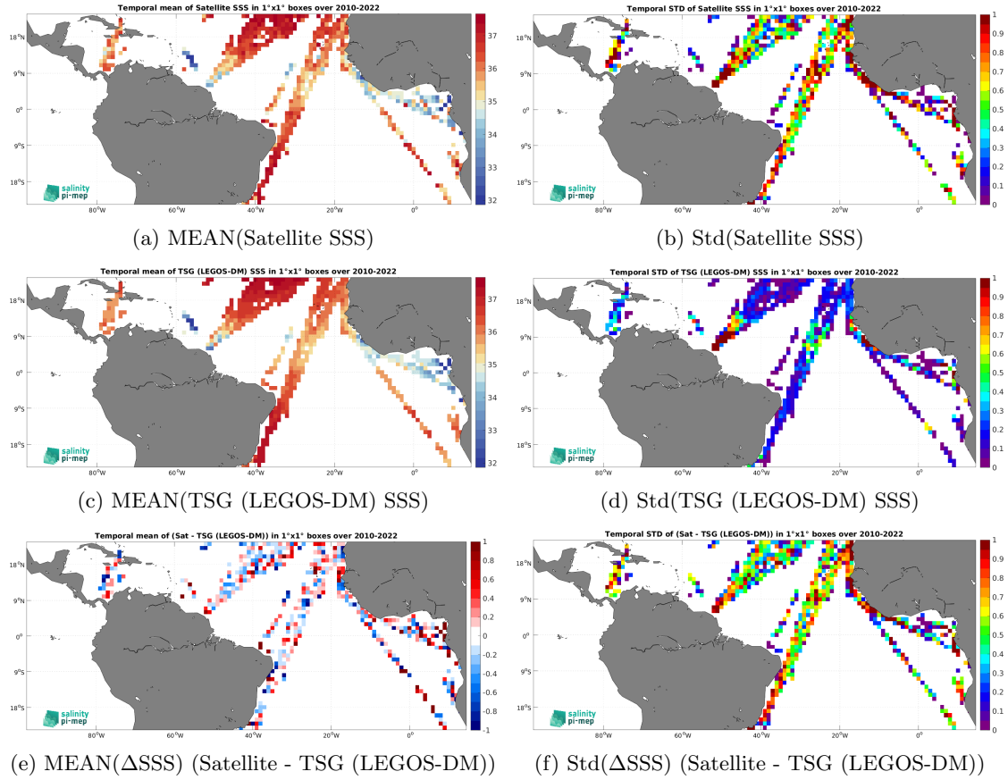
Figure 6: Temporal mean (left) and Std (right) of SSS from SMOS SSS L2Q v331 - 0.25 Deg (CATDS-CPDC) (top), TSG (LEGOS-DM) (middle), and of \Delta SSS (Satellite - TSG (LEGOS-DM)). Only match-up pairs are used to generate these maps.
