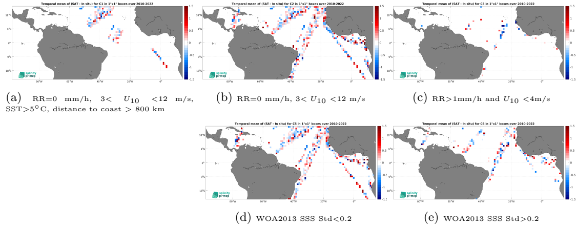
Figure 12: Temporal mean gridded over spatial boxes of size 1^{\circ}\times 1^{\circ} of \Delta\text{SSS} (SMOS SSS L2Q v331 - 0.25 Deg (CATDS-CPDC) - TSG (LEGOS-DM)) for 5 different subdatasets corresponding to: RR=0 mm/h, 3 < U_{10} < 12 m/s, SST > 5^{\circ}\text{C} , distance to coast > 800 km (a), RR=0 mm/h, 3 < U_{10} < 12 m/s (b), RR > 1 mm/h and U_{10} < 4 m/s (c), WOA2013 SSS Std < 0.2 (d), WOA2013 SSS Std > 0.2 (e).
