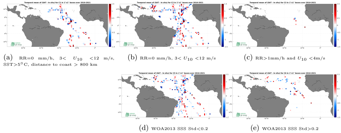
Figure 12: Temporal mean gridded over spatial boxes of size 1^{\circ}\times 1^{\circ} of \Delta SSS (SMOS SSS L2Q v331 - 0.25 Deg (CATDS-CPDC) - TSG (GOSUD-Sailing-ship)) for 5 different subdatasets corresponding to:RR=0 mm/h, 3 < U_{10} < 12 m/s, SST >5^{\circ}\text{C} , distance to coast > 800 km (a), RR=0 mm/h, 3 < U_{10} < 12 m/s (b), RR >1 mm/h and U_{10} < 4 m/s (c), WOA2013 SSS Std <0.2 (d), WOA2013 SSS Std >0.2 (e).
