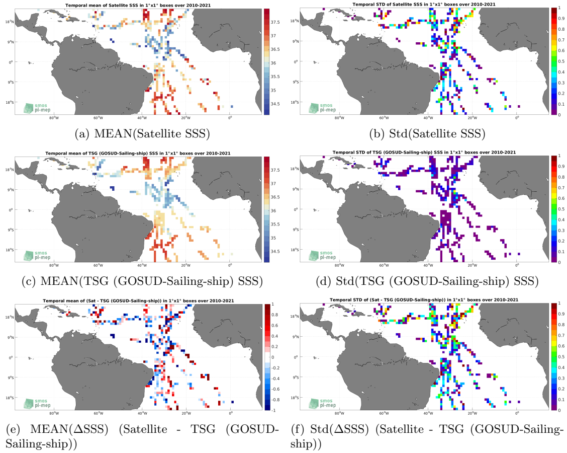
Figure 6: Temporal mean (left) and Std (right) of SSS from SMOS SSS L2Q v331 - 0.25 Deg (CATDS-CPDC) (top), TSG (GOSUD-Sailing-ship) (middle), and of \Delta SSS (Satellite - TSG (GOSUD-Sailing-ship)). Only match-up pairs are used to generate these maps.
