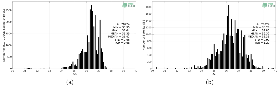
Figure 2: Histograms of SSS from TSG (GOSUD-Sailing-ship) (a) and SMOS SSS L2Q v331 - 0.25 Deg (CATDS-CPDC) (b) considering all match-up pairs per bins of 0.1 over the Tropical Atlantic Ocean Pi-MEP region and for the full satellite product period.
