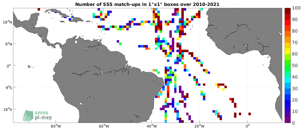
Figure 4: Number of SSS match-ups between TSG (GOSUD-Sailing-ship) SSS and the SMOS SSS L2Q v331 - 0.25 Deg (CATDS-CPDC) SSS product for the Tropical Atlantic Ocean Pi-MEP region over 1^\circ \times 1^\circ boxes and for the full satellite product period.
