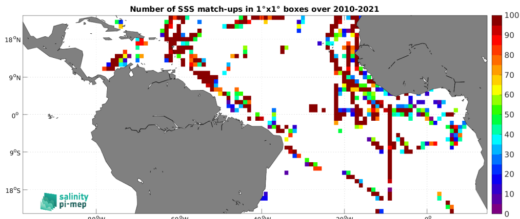
Figure 4: Number of SSS match-ups between TSG (GOSUD-Research-vessel) SSS and the SMOS SSS L2Q v331 - 0.25 Deg (CATDS-CPDC) SSS product for the Tropical Atlantic Ocean Pi-MEP region over 1^\circ \times 1^\circ boxes and for the full satellite product period.
