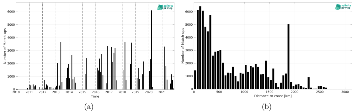
Figure 1: Number of match-ups between TSG (GOSUD-Research-vessel) and SMOS SSS L2Q v331 - 0.25 Deg (CATDS-CPDC) SSS as a function of time (a) and as function of the distance to coast (b) over the Tropical Atlantic Ocean Pi-MEP region and for the full satellite product period.
