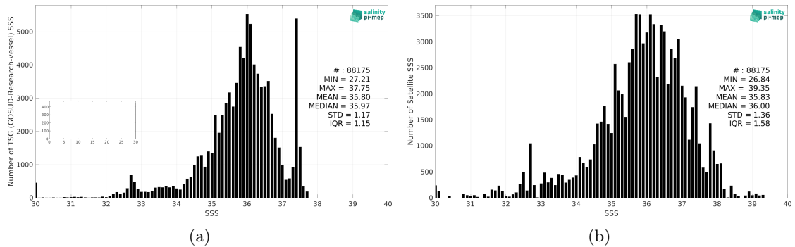
Figure 2: Histograms of SSS from TSG (GOSUD-Research-vessel) (a) and SMOS SSS L2Q v331 - 0.25 Deg (CATDS-CPDC) (b) considering all match-up pairs per bins of 0.1 over the Tropical Atlantic Ocean Pi-MEP region and for the full satellite product period.
