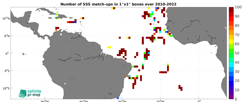
Figure 4: Number of SSS match-ups between TSG (CSIC-UTM) SSS and the SMOS SSS L2Q v331 - 0.25 Deg (CATDS-CPDC) SSS product for the Tropical Atlantic Ocean Pi-MEP region over 1^\circ \times 1^\circ boxes and for the full satellite product period.
