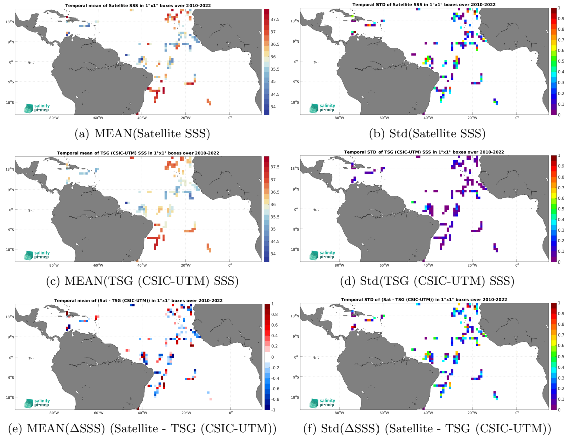
Figure 6: Temporal mean (left) and Std (right) of SSS from SMOS SSS L2Q v331 - 0.25 Deg (CATDS-CPDC) (top), TSG (CSIC-UTM) (middle), and of \Delta SSS (Satellite - TSG (CSIC-UTM)). Only match-up pairs are used to generate these maps.
