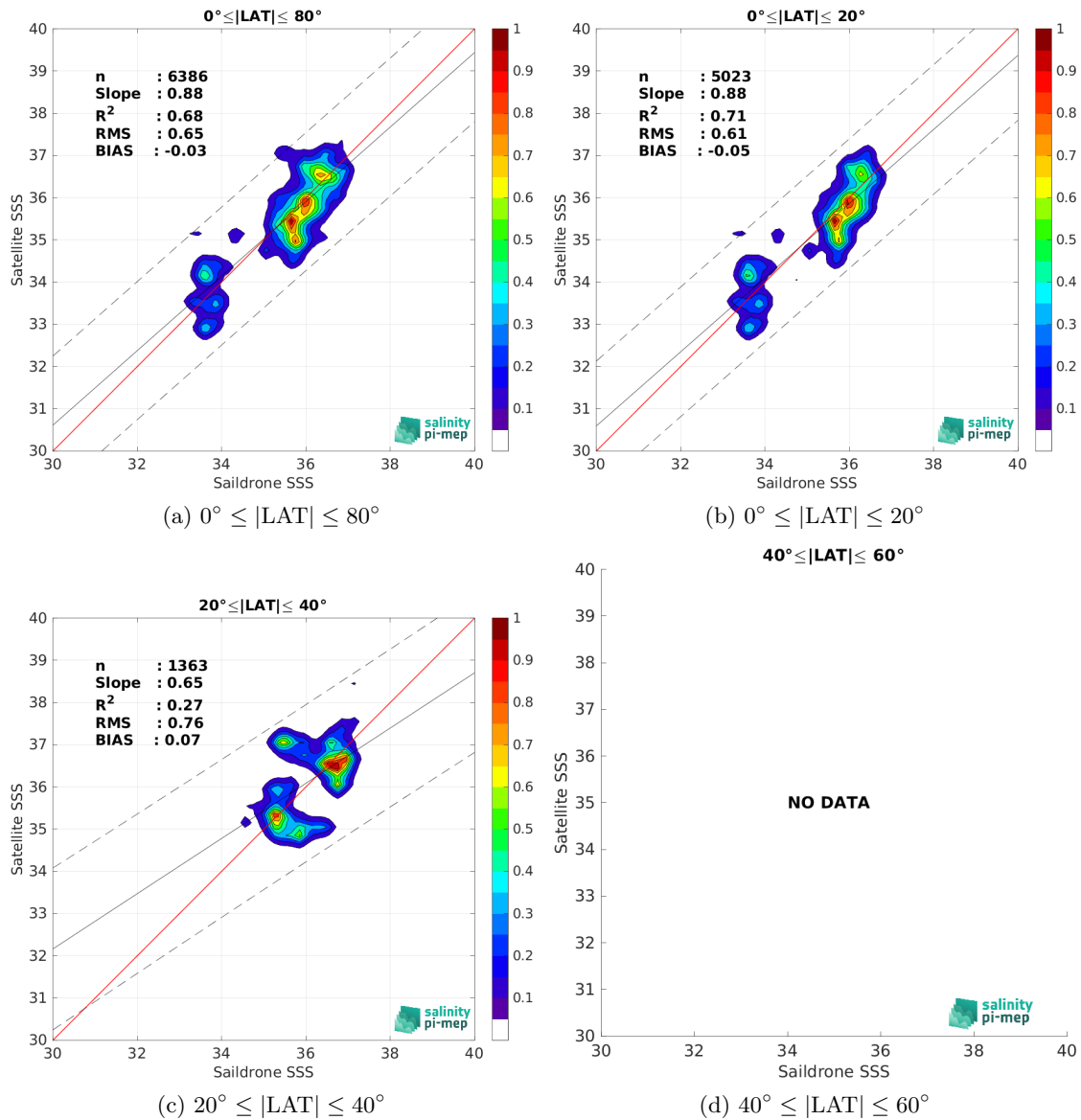
Figure 9: Contour maps of the concentration of SMOS SSS L2Q v331 - 0.25 Deg (CATDS-CPDC) SSS (y-axis) versus Saildrone SSS (x-axis) at match-up pairs for different latitude bands. For each plot, the red line shows x=y . The black thin and dashed lines indicate a linear fit through the data cloud and the \pm 95\% confidence levels, respectively. The number match-up pairs n , the slope and R^2 coefficient of the linear fit, the root mean square (RMS) and the mean bias between satellite and in situ data are indicated for each latitude band in each plots.
