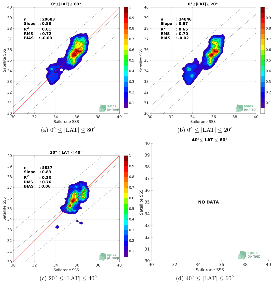
Figure 9: Contour maps of the concentration of SMOS SSS L2Q v331 - 0.25 Deg (CATDS-CPDC) SSS (y-axis) versus Sailldrone SSS (x-axis) at match-up pairs for different latitude bands. For each plot, the red line shows x=y . The black thin and dashed lines indicate a linear fit through the data cloud and the \pm 95\% confidence levels, respectively. The number match-up pairs n , the slope and R^2 coefficient of the linear fit, the root mean square (RMS) and the mean bias between satellite and in situ data are indicated for each latitude band in each plots.
