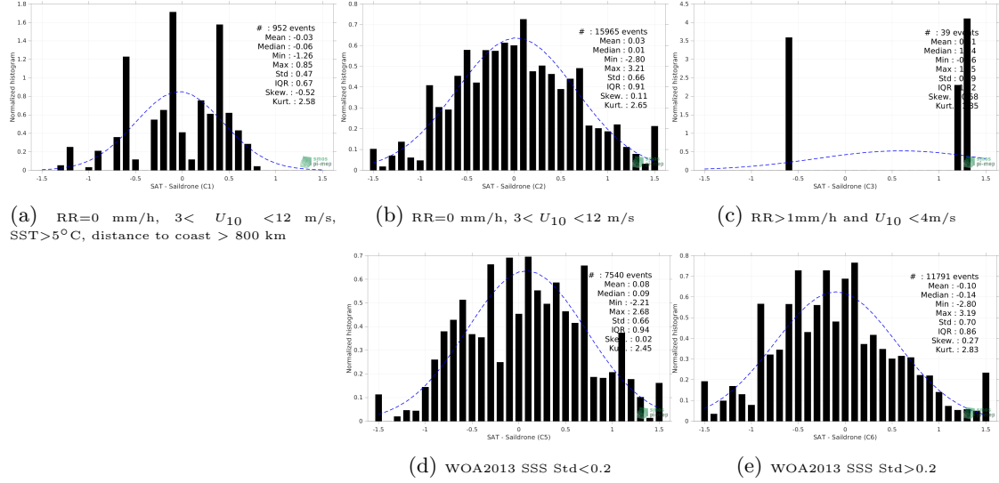
Figure 13: Normalized histogram of \Delta SSS (SMOS SSS L2Q v331 - 0.25 Deg (CATDS-CPDC) - Saildrone) for 5 different subdatasets corresponding to: RR=0 mm/h, 3 < U_{10} < 12 m/s, SST>5°C, distance to coast > 800 km (a), RR=0 mm/h, 3 < U_{10} < 12 m/s (b), RR>1mm/h and U_{10} < 4 m/s (c), WOA2013 SSS Std<0.2 (d), WOA2013 SSS Std>0.2 (e).
