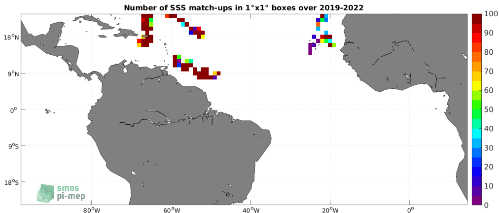
Figure 4: Number of SSS match-ups between Saildrone SSS and the SMOS SSS L2Q v331 - 0.25 Deg (CATDS-CPDC) SSS product for the Tropical Atlantic Ocean Pi-MEP region over 1^\circ \times 1^\circ boxes and for the full satellite product period.
