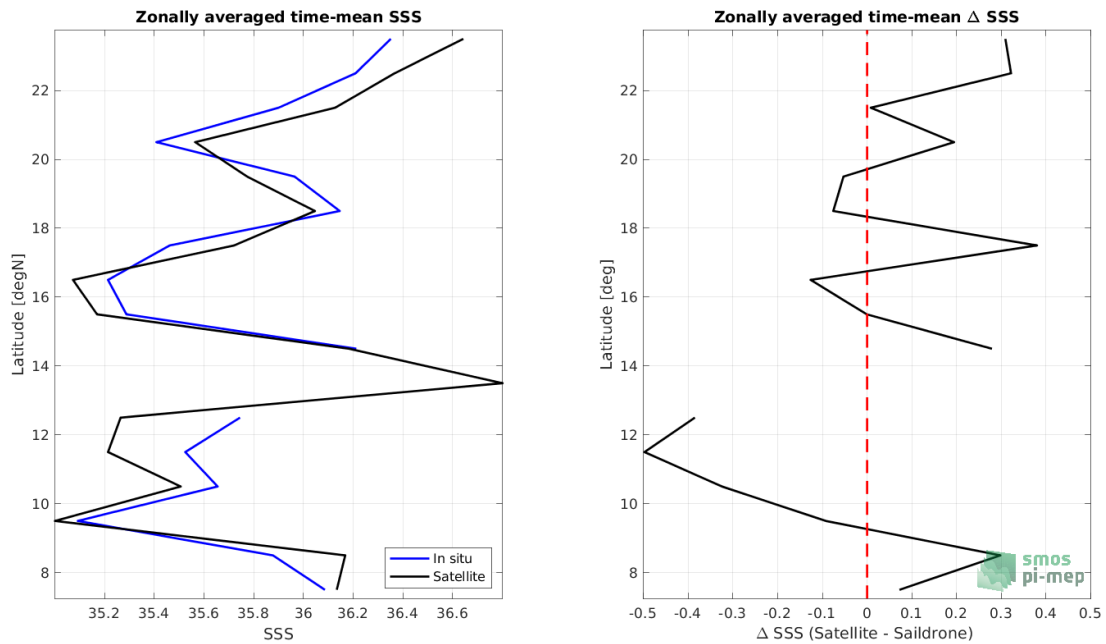
Figure 8: Left panel: Zonal mean SSS from SMOS SSS L2Q v331 - 0.25 Deg (CATDS-CPDC) satellite product (black) and from Sairdrone (blue). Right panel: Zonal mean of \Delta SSS (Satellite - Sairdrone) for all the collected Pi-MEP match-up pairs estimated over the full satellite product period.
