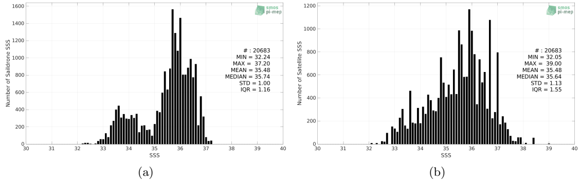
Figure 2: Histograms of SSS from Saildrone (a) and SMOS SSS L2Q v331 - 0.25 Deg (CATDS-CPDC) (b) considering all match-up pairs per bins of 0.1 over the Tropical Atlantic Ocean Pi-MEP region and for the full satellite product period.
