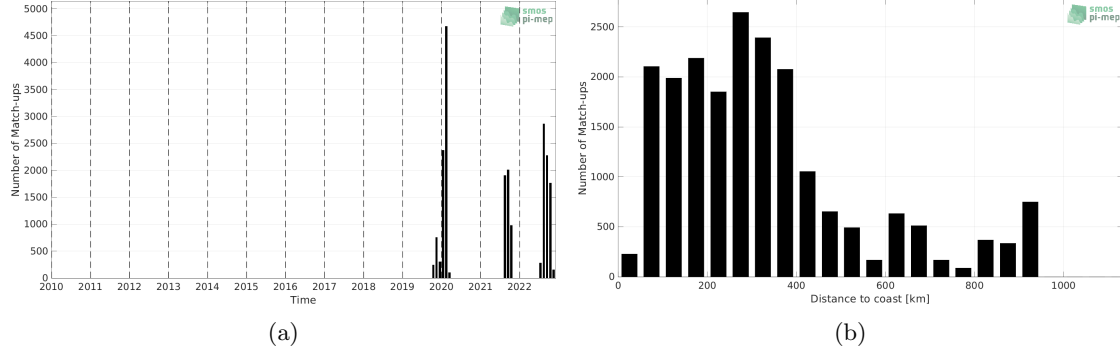
Figure 1: Number of match-ups between Saildrone and SMOS SSS L2Q v331 - 0.25 Deg (CATDS-CPDC) SSS as a function of time (a) and as function of the distance to coast (b) over the Tropical Atlantic Ocean Pi-MEP region and for the full satellite product period.
