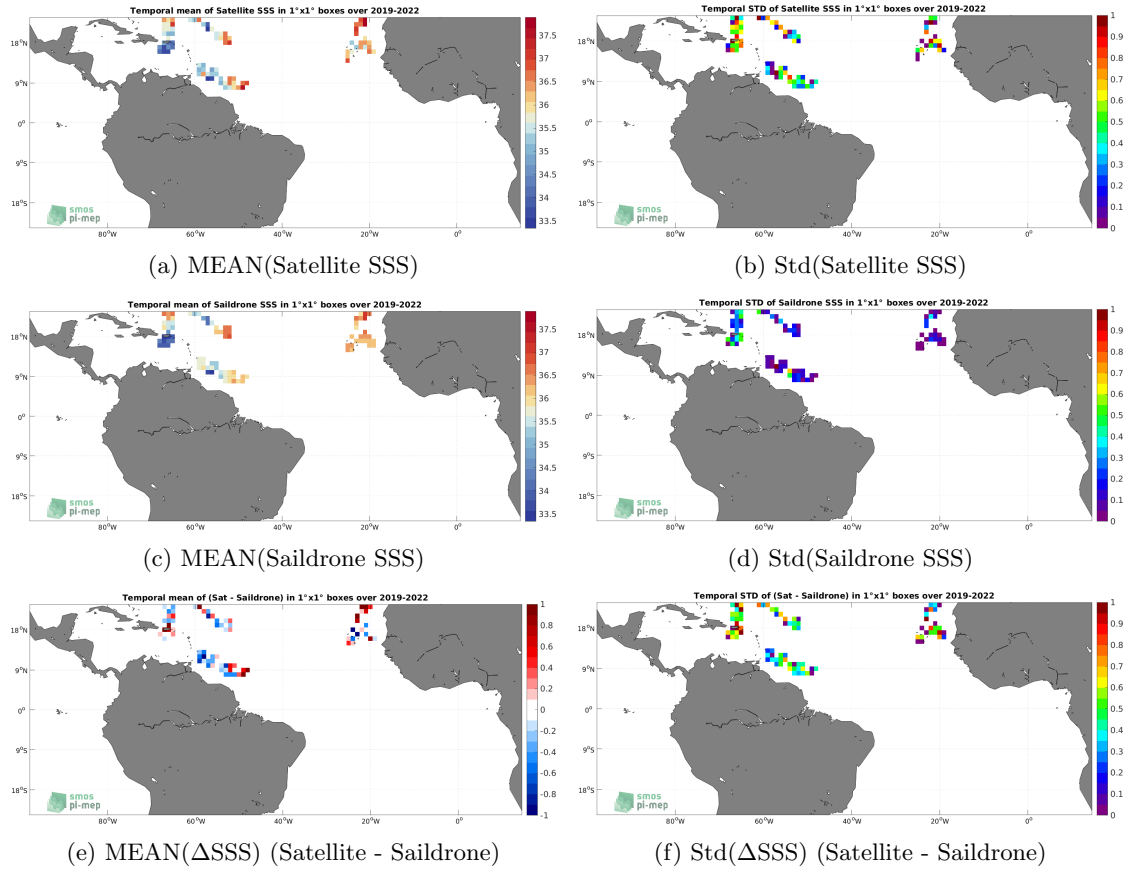
Figure 6: Temporal mean (left) and Std (right) of SSS from SMOS SSS L2Q v331 - 0.25 Deg (CATDS-CPDC) (top), Saildrone (middle), and of \Delta SSS (Satellite - Saildrone). Only match-up pairs are used to generate these maps.
