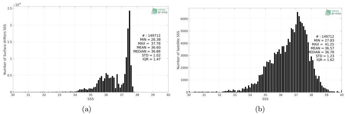
Figure 2: Histograms of SSS from Surface drifters (a) and SMOS SSS L2Q v331 - 0.25 Deg (CATDS-CPDC) (b) considering all match-up pairs per bins of 0.1 over the Tropical Atlantic Ocean Pi-MEP region and for the full satellite product period.
