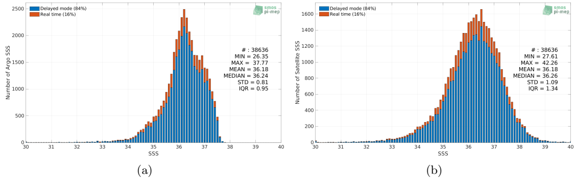
Figure 2: Histograms of SSS from Argo (a) and SMOS SSS L2Q v331 - 0.25 Deg (CATDS-CPDC) (b) considering all match-up pairs per bins of 0.1 over the Tropical Atlantic Ocean Pi-MEP region and for the full satellite product period.
