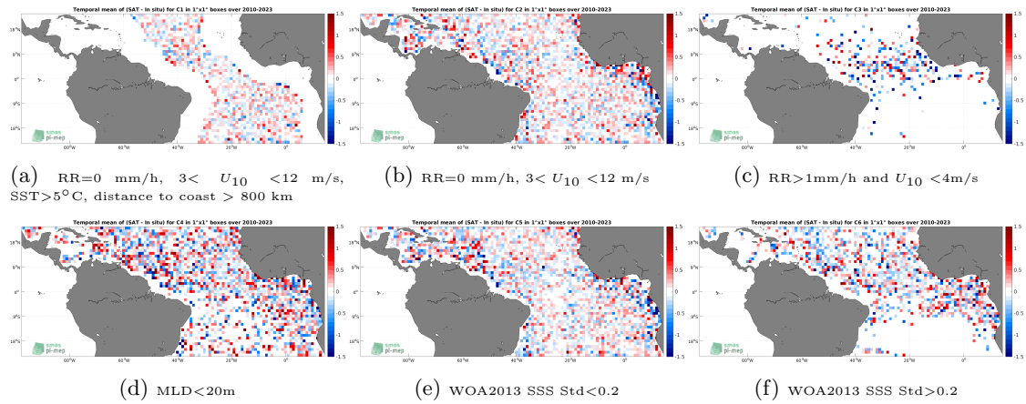
Figure 12: Temporal mean gridded over spatial boxes of size 1^\circ \times 1^\circ of \Delta SSS (SMOS SSS L2Q v331 - 0.25 Deg (CATDS-CPDC) - Argo) for 6 different subdatasets corresponding to:RR=0 mm/h, 3 < U_{10} < 12 m/s, SST >5^\circ C, distance to coast > 800 km (a), RR=0 mm/h, 3 < U_{10} < 12 m/s (b), RR >1 mm/h and U_{10} < 4 m/s (c),MLD <20 m (d),WOA2013 SSS Std <0.2 (e),WOA2013 SSS Std >0.2 (f).
