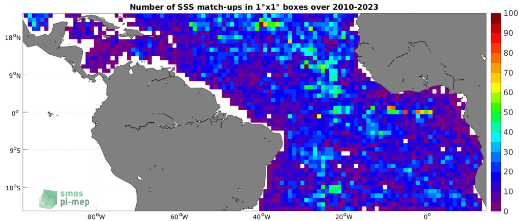
Figure 4: Number of SSS match-ups between Argo SSS and the SMOS SSS L2Q v331 - 0.25 Deg (CATDS-CPDC) SSS product for the Tropical Atlantic Ocean Pi-MEP region over 1^\circ \times 1^\circ boxes and for the full satellite product period.
