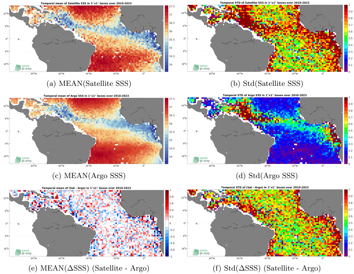
Figure 6: Temporal mean (left) and Std (right) of SSS from SMOS SSS L2Q v331 - 0.25 Deg (CATDS-CPDC) (top), Argo (middle), and of \Delta SSS (Satellite - Argo). Only match-up pairs are used to generate these maps.
