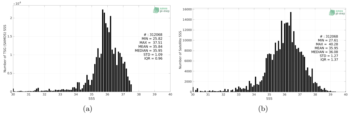
Figure 2: Histograms of SSS from TSG (SAMOS) (a) and SMOS SSS L2Q v330 - 0.25 Deg (CATDS-CPDC) (b) considering all match-up pairs per bins of 0.1 over the Tropical Atlantic Ocean Pi-MEP region and for the full satellite product period.
