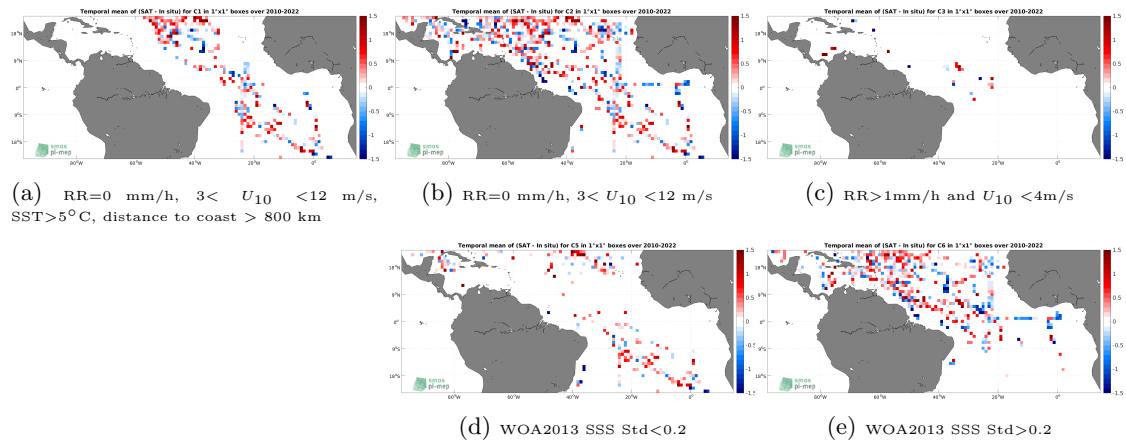
Figure 12: Temporal mean gridded over spatial boxes of size 1^\circ \times 1^\circ of \Delta SSS (SMOS SSS L2Q v330 - 0.25 Deg (CATDS-CPDC) - TSG (SAMOS)) for 5 different subdatasets corresponding to:RR=0 mm/h, 3 < U_{10} < 12 m/s, SST >5^\circ C, distance to coast > 800 km (a), RR=0 mm/h, 3 < U_{10} < 12 m/s (b), RR >1 mm/h and U_{10} < 4 m/s (c), WOA2013 SSS Std <0.2 (d), WOA2013 SSS Std >0.2 (e).
