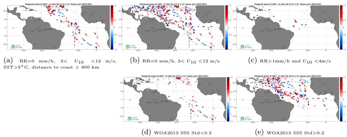
Figure 12: Temporal mean gridded over spatial boxes of size 1^\circ \times 1^\circ of \Delta SSS (SMOS SSS L2Q v321 - 0.25 Deg (CATDS-CPDC) - TSG (SAMOS)) for 5 different subdatasets corresponding to:RR=0 mm/h, 3 < U_{10} < 12 m/s, SST >5^\circ C, distance to coast > 800 km (a), RR=0 mm/h, 3 < U_{10} < 12 m/s (b), RR >1 mm/h and U_{10} < 4 m/s (c), WOA2013 SSS Std <0.2 (d), WOA2013 SSS Std >0.2 (e).
